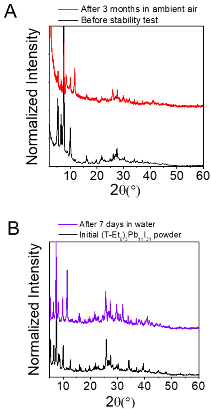
Figure 4. (A) PXRD pattern of (T-Et 6 ) 3 Pb 11 I 31 crystals before and after 3 months stored in ambient air. (B) PXRD pattern of (T-Et 6 ) 3 Pb 11 I 31 crystals before and after 7 days in water.
