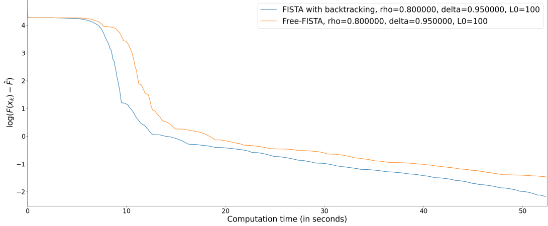
Figure 13: Convergence rates in function values VS. CPU time for problem (4.5).
