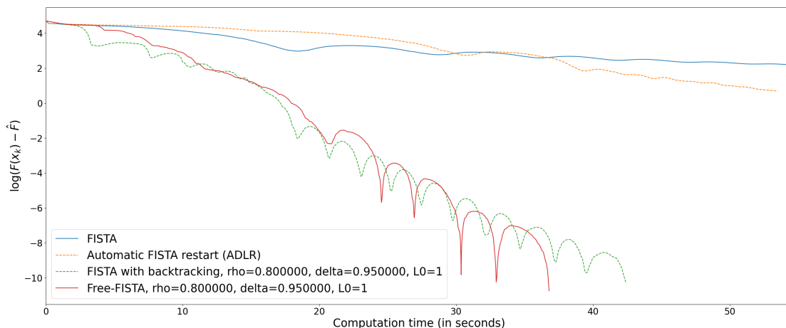
Figure 2: Convergence rates w.r.t. CPU times for problem (4.1).
