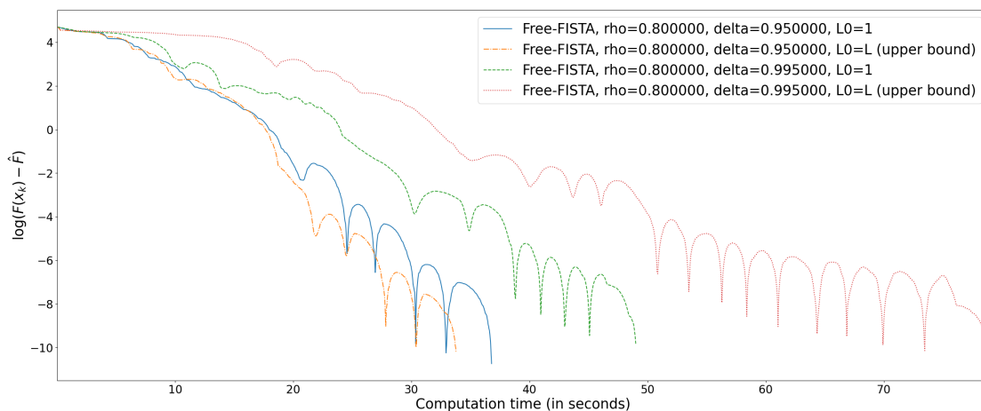
Figure 3: Convergence rates of Free-FISTA for several choices of parameters \rho , \delta and L_0 w.r.t. CPU time for problem (4.1).
