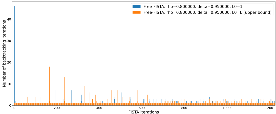
Figure 5: Number of backtracking calls per total FISTA iterations for problem (4.1).
