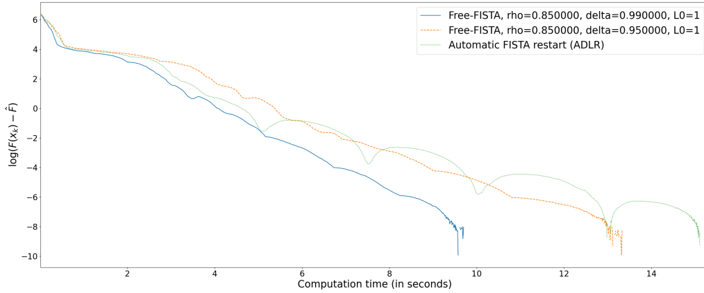
Figure 10: Convergence rates in function values w.r.t the CPU time for problem (4.3).
