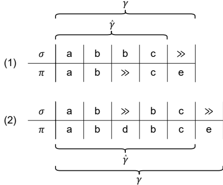
Figure 2: Running example: two optimal alignments and prefix-alignments.
