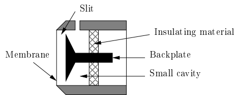
Figure 1: Condenser microphone.
