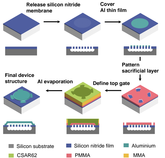
Fig. 1. Schematic of nanofabrication process for a silicon nitride drum nanoelectromechanical resonator. It includes the dry etching process to release the membrane from the substrate, the deposition of a metal layer on the surface of the membrane and the two-step lithography process to create a suspended top gate.
