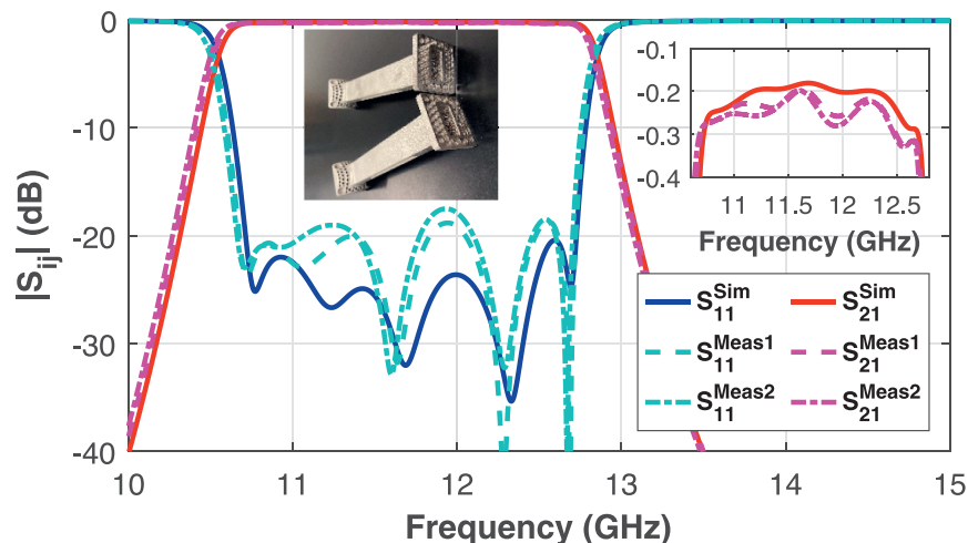
Figure 6. Simulated and measured scattering parameters of an evanescent mode filter with chamfered ridges. Two copies of the prototype have been manufactured in order to assess the repeatability. These figures are shown here for the first time.
