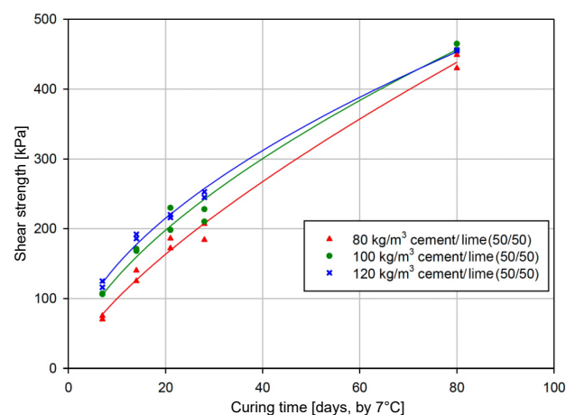
Fig. 10. Shear strength as a function of curing time for test specimens stabilized by a combination of CEM II/A and burned lime (50/50).
