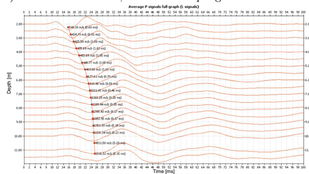
c) Borehole: ACW151, z -direction – p -signal
