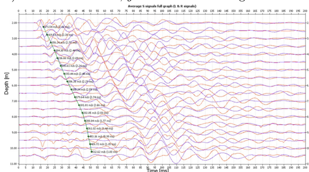
b) Borehole: ADA147, y -direction – mean signal
