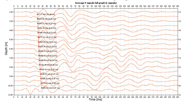
Fig. 18. Signals for ADC148 column.
