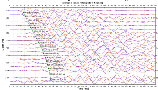
b) Borehole: ACW151, y -direction – mean signal
