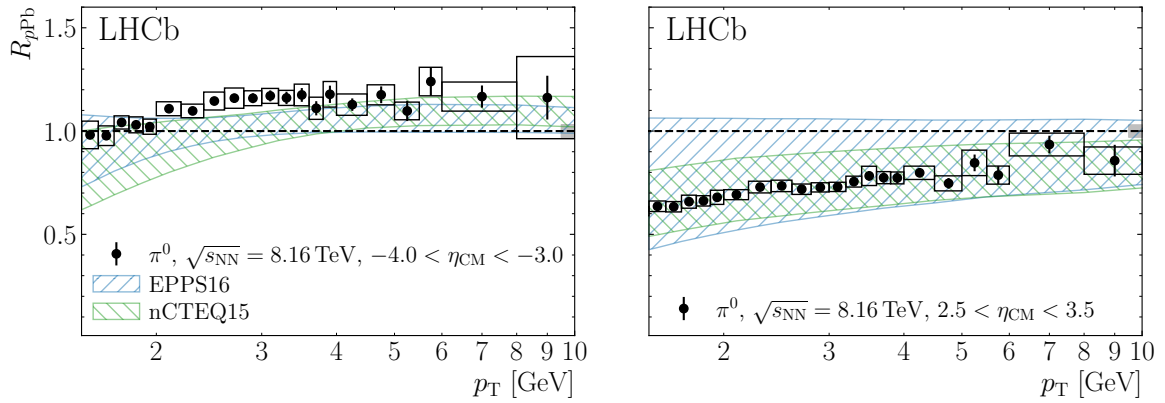
Figure S1: Measured \pi^0 nuclear modification factor in the (left) backward and (right) forward \eta_{\text{CM}} regions. The error bars show the statistical uncertainties, while the open boxes show the p_{\text{T}} -dependent systematic uncertainties. The solid black boxes show the overall normalization uncertainties from the luminosity estimate and efficiency correction factors. The measurements are compared to NLO PQCD predictions [47] calculated using the EPPS16 [2] and nCTEQ15 [3] NPDF sets.
