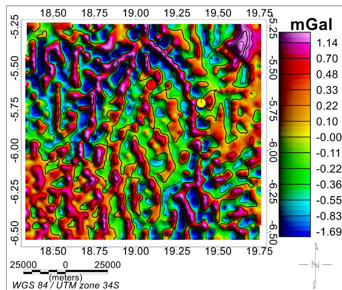
Figure 7. Residual anomalies in our study area. Kakobola in red circle and Gungu in yellow circle.
