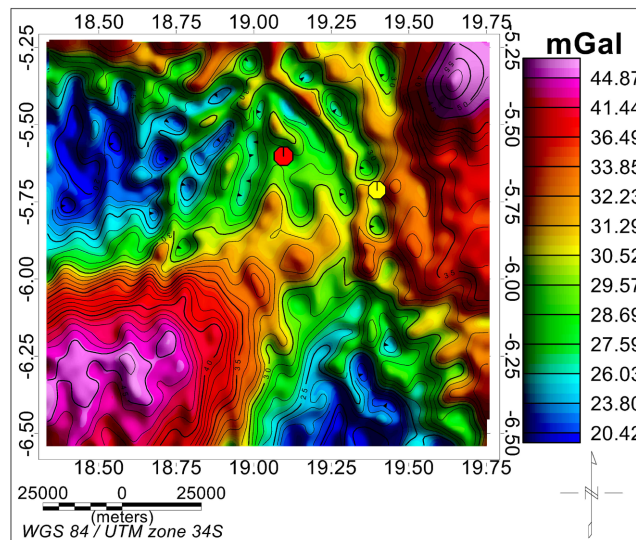
Figure 5. Regional gravity anomalies from the upward continuation of the CBAs at 1000 m elevation. Kakobola in red circle and Gungu in yellow circle.
