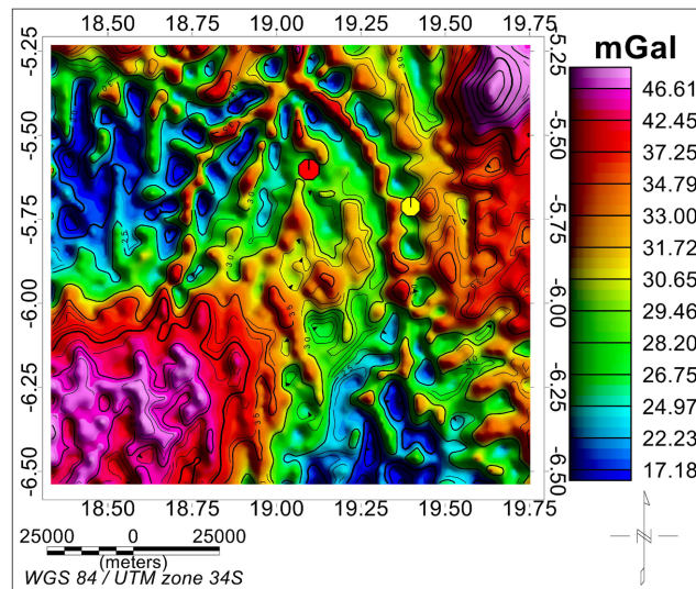
Figure 4. Complete Bouguer anomalies from our study area. Kakobola in red circle and Gungu in yellow circle.
