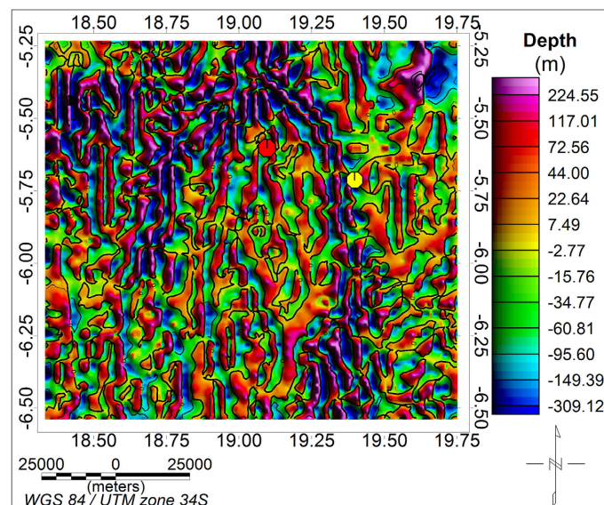
Figure 9. Depth of the subsurface source anomalies in our study area from tilt angle. Kakobola in red circle and Gungu in yellow circle.
