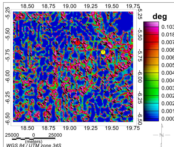
Figure 12. Dip map of the CBAs in our study area. Kakobola in red circle and Gungu in yellow circle.
