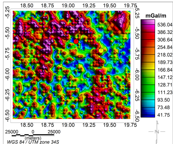
Figure 10. Analytical signal of the CBAs in our study area. Kakobola in red circle and Gungu in yellow circle.
