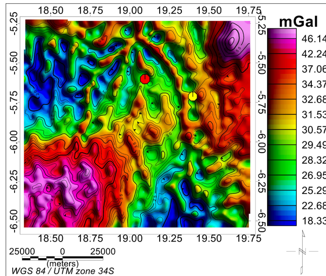
Figure 6. Regional anomalies from the upward continuation of the CBAs at 500 m elevation. Kakobola in red circle and Gungu in yellow circle.
