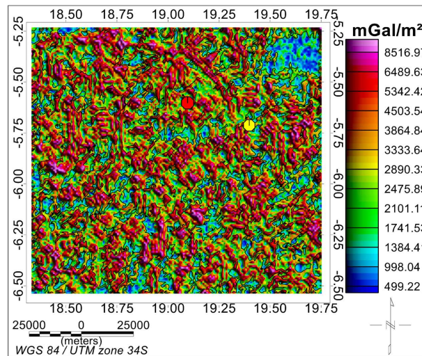
Figure 11. FTHTD of the CBAs in our study area. Kakobola in red circle and Gungu in yellow circle.
