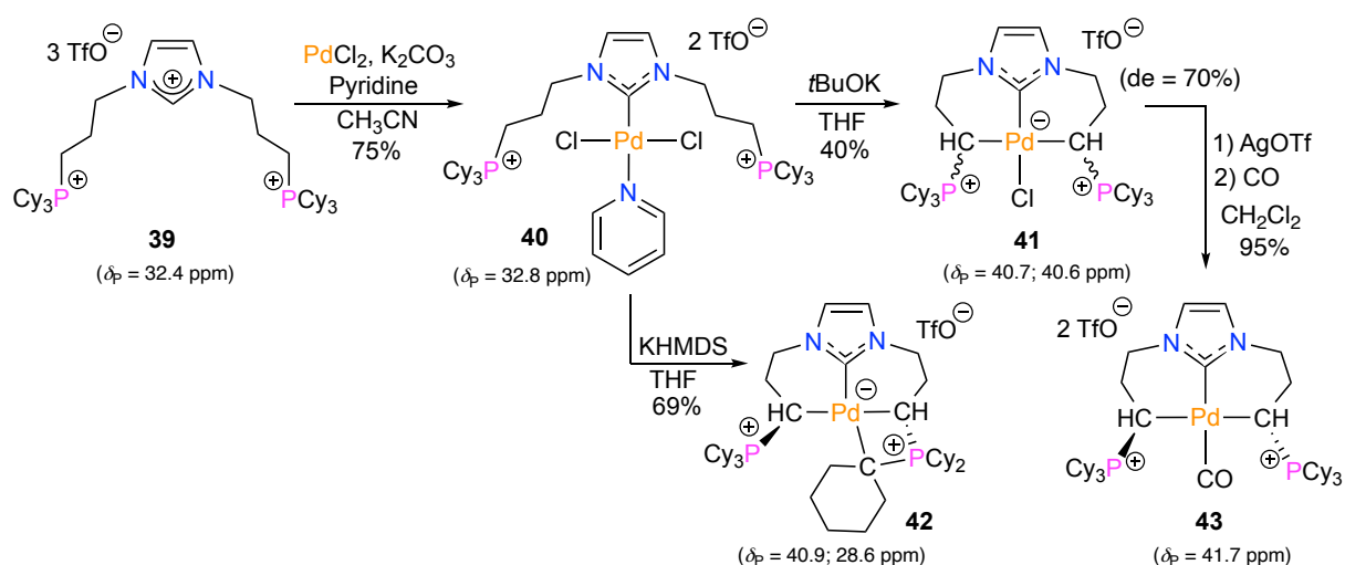
Scheme 18. Preparation of NHC core, diphosphonium bis(ylide) Pd(II) pincer complexes 41-43 from the imidazolium salt 39 (in the \text{PCy}_3^+ series). [50]
