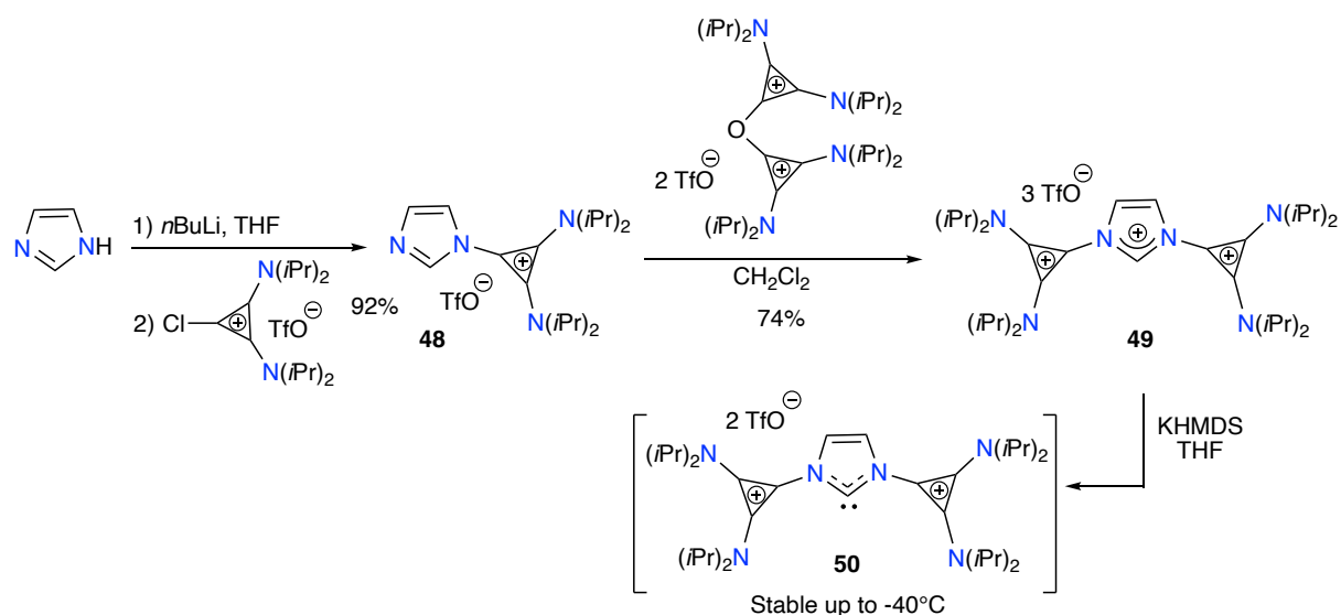
Scheme 21. Preparation of the imidazolium salt 49 from 1 H -imidazole with 13 C NMR identification of corresponding dicationic NHC 50 . [52]
