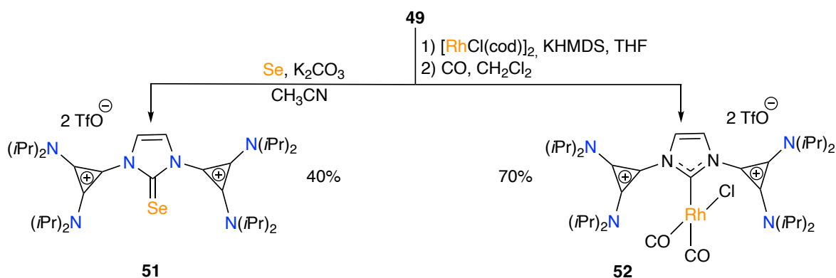
Scheme 22. Syntheses of the selenourea 51 and NHC Rh I complex 52 from imidazolium salt 49 . [52]
