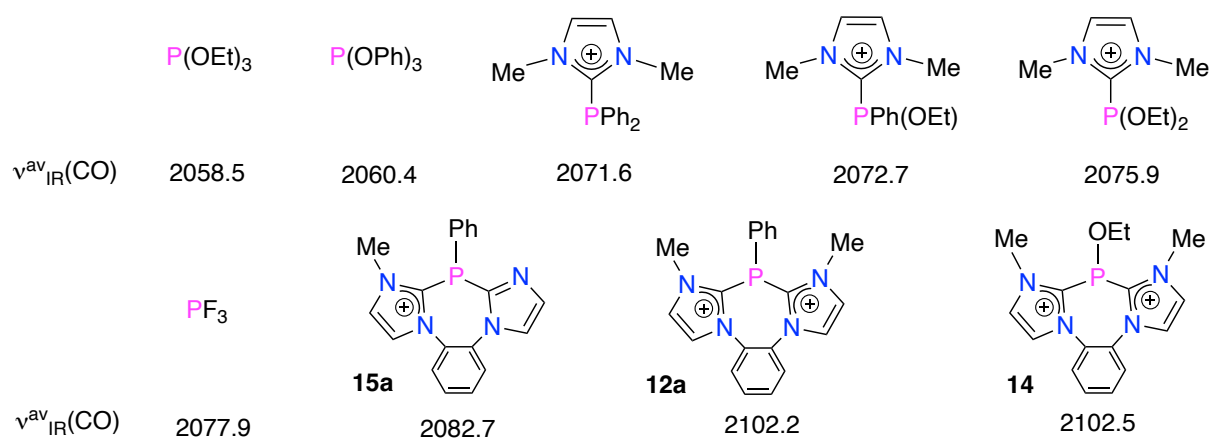
Scheme 10. Comparative scale of the electron-donating ability of electron-poor phosphorus ligands L based on the average of calculated IR \nu_{CO} stretching frequencies (in cm^{-1} ) in [Rh(L)(CO)_2Cl] complexes. [31]
