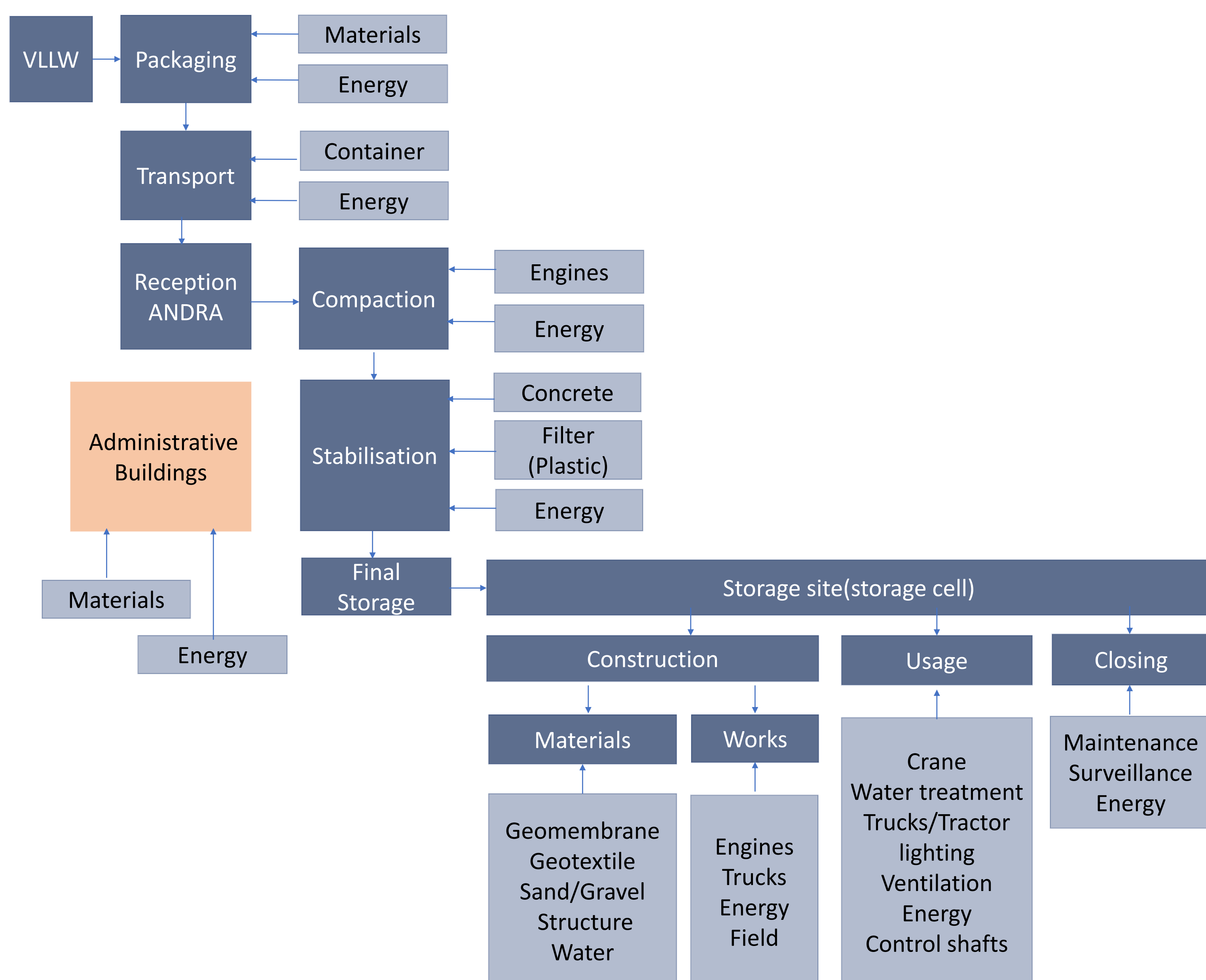
Figure 2 : System boundary diagram representing the storage scenario made by Zineb GUENDOZ
