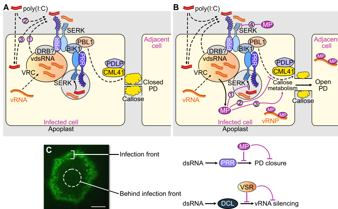
Figure 10. Virus infection facilitated by virus-encoded effector proteins. A and B ) Suppression of PTI by MP. A ) Perception of dsRNA produced in cortical ER-associated VRCs at the PM by an unknown membrane-associated or intracellular PRR and the SERK1 coreceptor (with potential contribution by one or more other coreceptors) triggers a signaling pathway leading to callose deposition and PD closure. dsRNA produced during infection in the VRC may require secretion into the apoplast (1) to allow perception at the PM. Externally applied poly(I:C) may be perceived from the apoplast (2) or secreted upon initial uptake by the cells (3). Viral dsRNA as well as poly(I:C) may also be sensed by an intracellular cytoplasmic PRR, or by an internalized SERK–PRR complex, as shown in the figure in endosomes, shown as a gray vesicle. B ) MP suppresses dsRNA-triggered callose deposition and allows intercellular spread of the viral ribonucleoprotein complex (vRNP). The MP may inhibit dsRNA sensing by the intracellular dsRNA receptor or internalized SERK–PRR complex (1), interact with intracellular PTI signaling (2) or modify the activity of callose synthesizing or degrading enzymes at PD (3). The MP may also be secreted to inhibit dsRNA perception at the PM (4). C ) dsRNA triggers PTI and antiviral RNA silencing and both responses are suppressed by viral effector proteins to support virus propagation. Whereas MP acts in cells at the virus front to facilitate virus movement by blocking a dsRNA-induced callose defense response at PD, the VSR blocks dsRNA-induced antiviral RNA silencing in the center of infection sites to support virus replication and production of virus progeny. A local infection site of TMV encoding MP fused to GFP (TMV-MP:GFP, 7 dpi) in N. benthamiana is shown. Scale bar, 1 mm.
