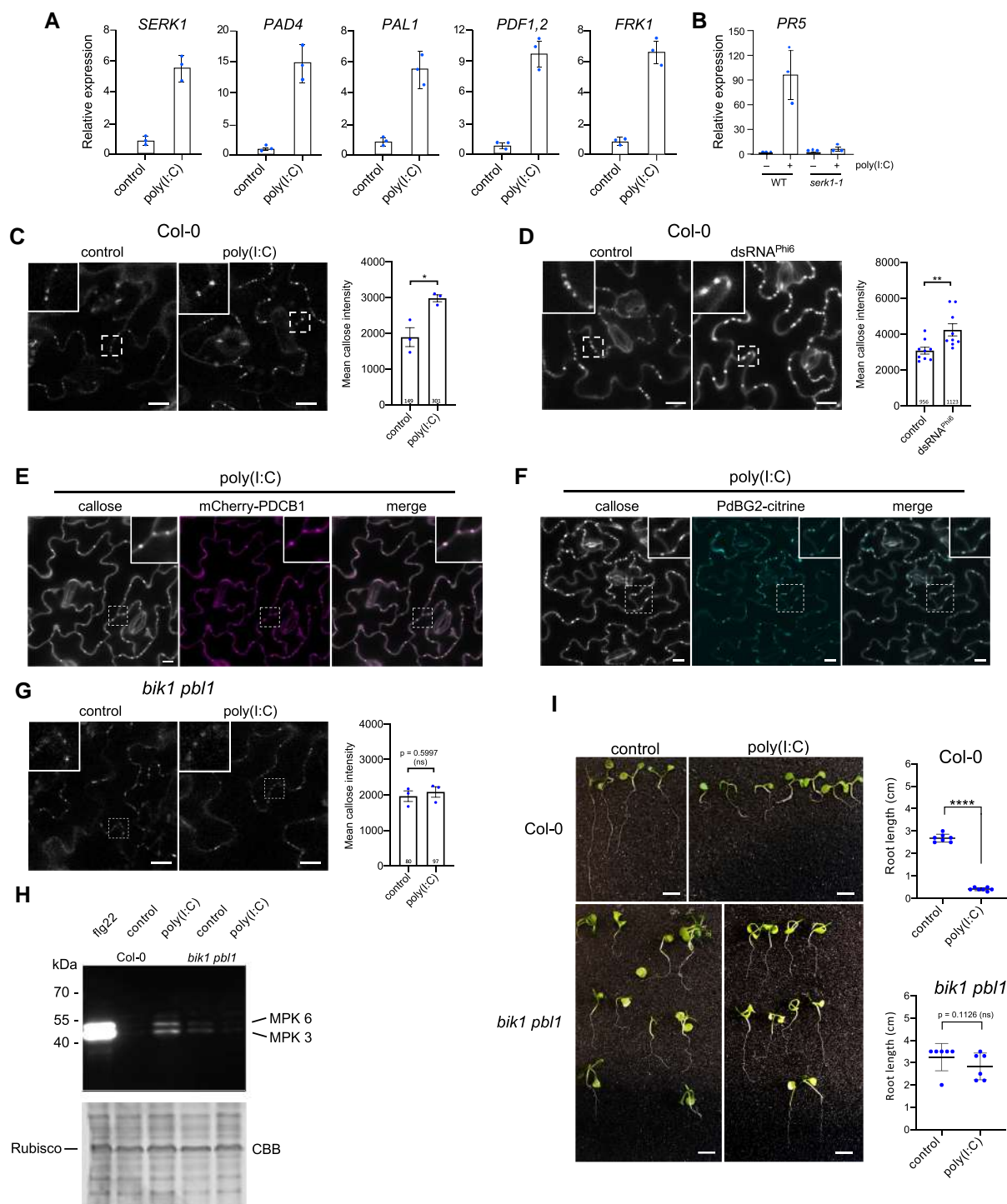
Figure 2. Poly(I:C)-induced signaling in Arabidopsis depends on BIK1/PBL1. A and B ) Transcriptional regulation of Arabidopsis genes 3 h after treatment with 0.5 \mu\text{g}/\mu\text{L} poly(I:C). For each gene, the mean value and the standard deviation of gene expression values obtained by RT-qPCR analysis of 3 biological replicates (dots) is shown. A ) Poly(I:C) induces innate immunity marker genes in A. thaliana Col-0 wildtype. B ) Absence of poly(I:C)-induced PR5 expression in the serk1-1 mutant. C ) Poly(I:C) treatment causes callose deposition at PD in A. thaliana Col-0. Images were taken 30 min after treatment. Inlays show enlargements of the areas within the dashed boxes. Scale bar, 20 \mu\text{m} . Mean callose content in PD determined in 3 leaf disks from 3 plants per treatment (dots). The total number of evaluated PD is given at the base of each column. Error bars show the SEM. Two-tailed t -test; *, P = <0.05 . D ) Callose deposition at PD in A. thaliana Col-0 leaf epidermal tissue 30 min after treatment with 50 \text{ng}/\mu\text{L} of biological dsRNA (dsRNA Ph6 ). Inlays show enlargements of the areas within the dashed boxes. Scale bar, 20 \mu\text{m} . Mean callose content in PD determined in 9 leaf disks from 3 plants per treatment (dots). The total number of evaluated PD is given at the base of each column. Error bars show the SEM. Two-tailed t -test; **, P = <0.01 . E and F ) Poly(I:C)-induced callose spots are localized to PD as shown by colocalization with PD markers mCherry-PDCB1 E ) and PdBG2-citrine F ). Inlays show enlargements of the areas within the dashed boxes. Scale bar, 10 \mu\text{m} . G ) poly(I:C)-induced (continued)
