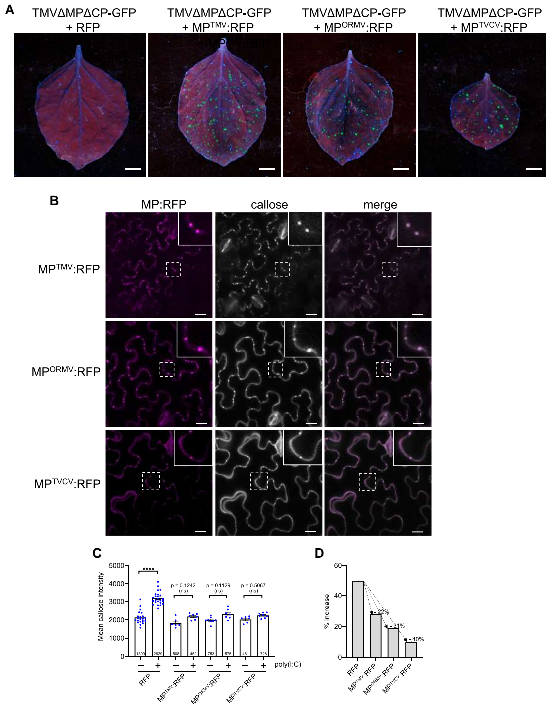
Figure 8. Inhibition of poly(l:C)-induced callose deposition by MPs of different viruses. A ) Different MPs are functional. Unlike free RFP, RFP fusions to the MPs of TMV (MP TMV :RFP), ORMV (MP ORMV :RFP), and TVCV (MP TVCV :RFP) complement the movement function of MP-deficient TMV \Delta M-GFP in N. benthamiana . Leaves were coinfiltrated with agrobacteria containing the respective RFP or MP:RFP-encoding plasmids together with highly diluted agrobacteria ( OD_{600\text{ nm}} = 1 \times 10^{-5} ) for agro-inoculation with TMV \Delta MP \Delta CP-GFP. Pictures were taken at 5 dpi. Scale bar, 1 cm. B ) MP TMV :RFP, MP ORMV :RFP, and MP TVCV :RFP localize to PD as shown by the presence of callose. MP-expressing leaves were stained with aniline blue and imaged after 30 min. Inlay images show magnifications of image areas framed by a dashed line. Scale bar, 20 \mu m. C and D ) Expression of either MP TMV :RFP, MP ORMV :RFP, or MP TVCV :RFP strongly reduces the induction of PD callose deposition in the presence of poly(l:C). Leaf disks excised from the RFP (control) or MP:RFP-expressing leaves 48 h after agroinfiltration were incubated for 1 d in water, then transferred into aniline blue solution with and without 0.5 \mu g/ \mu L poly(l:C) and imaged after 30 min. C ) Mean callose content in PD of poly(l:C)-treated and control-treated
