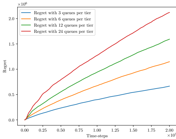
Figure 4: Regret of the UCRL-M algorithm on the queueing network for different values of n and scaling parameters.
