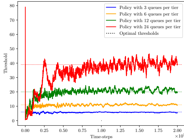
Figure 5: Average threshold chosen as a function of time.
