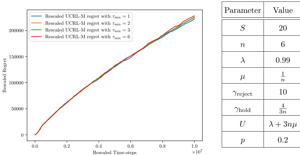
Figure 6: Rescaled regret of the UCRL-M algorithm on the queueing network for different values of \tau_{\text{mix}} .
