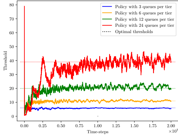
Figure 5: Average threshold chosen as a function of time.
