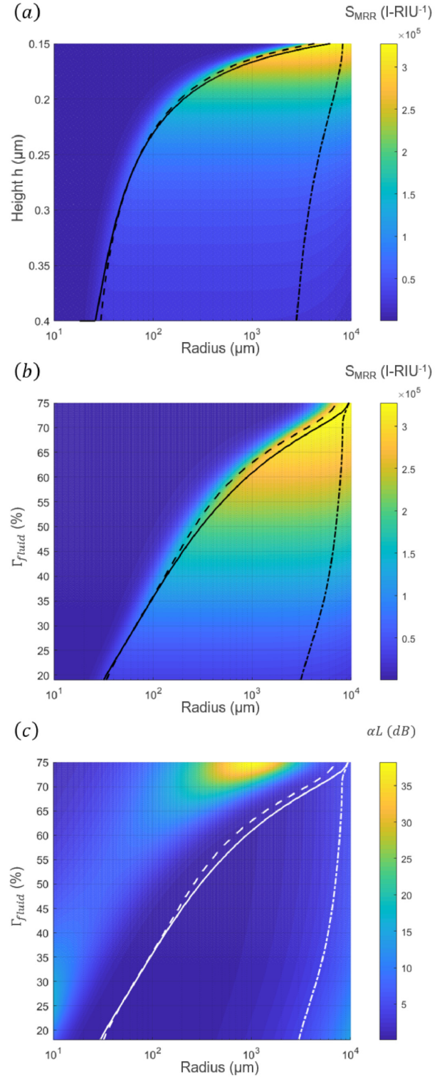
Fig. 5. (a) Sensitivity, S_{MRR} , as a function of waveguide core height versus ring radius; (b) Sensitivity and (c) round trip losses, \alpha L , as a function of evanescent field ratio versus ring radius. The solid curves trace the value pairs for (h, R) in (a) and (\Gamma_{fluid}, R) in (b) and (c) yielding the highest sensitivities. The dashed curves on either side indicate values of R_e (left) and R_{NR} (right) as a function of h and \Gamma_{fluid} . Waveguide core width = 0.7 \mu\text{m} .
