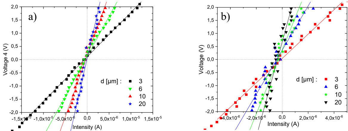
Fig. 7. I-V measurements of SiC sputtered PVD layers deposited at RT (a) and 400°C (b).
