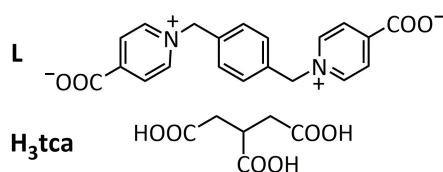
Scheme 1 The ligands L and H 3 tca.
