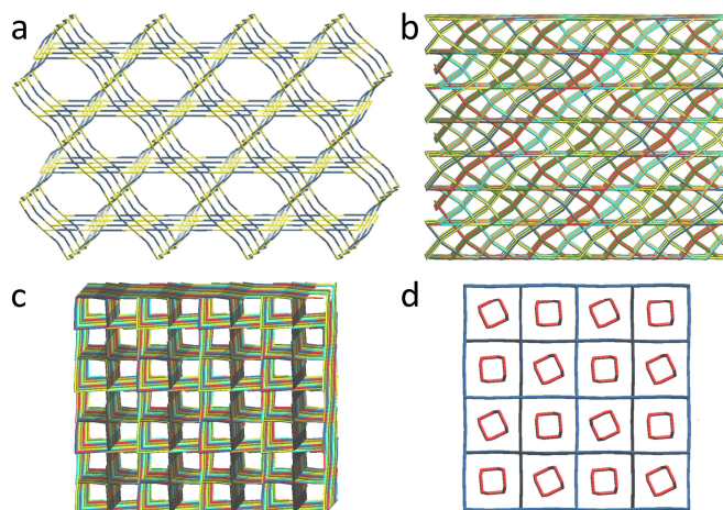
Fig. 2 (a) Nodal representation of a single network with 1vt topology in 1 down a direction slightly rotated from [103] (yellow, U nodes; blue, L edges). (b) and (c) Two views of the six-fold interpenetrated networks, down a direction slightly rotated from [100] or [001], respectively. (d) Nanotubes (red) included in the channels of the framework (blue), viewed down [001].
