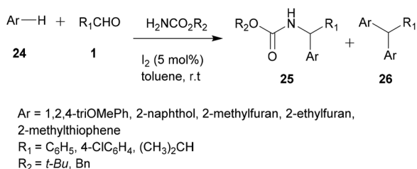
Scheme 6 One-pot three-component aza-FC reaction catalyzed by iodine.
