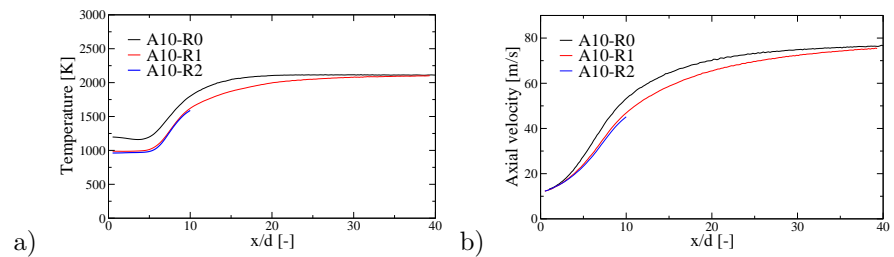
Fig. 17 Cases A10-R, mesh convergence. Transversally averaged (a) temperature and (b) axial velocity.
