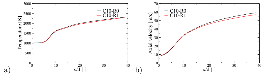
Fig. 12 Cases C10-R, mesh convergence. Transversally averaged (a) temperature and (b) axial velocity.
