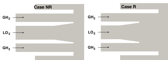
Fig. 2 Longitudinal cut of the coaxial injector (here shown for case C60). Left: non recessed injector ; right: recessed injector.
