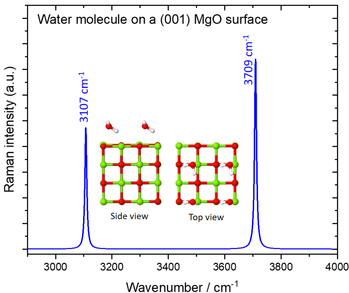
Figure 2. Calculated configuration and Raman spectra for a (001) MgO surface. Green balls corresponds to Mg atoms, red balls to O atoms and white balls to H atoms.
