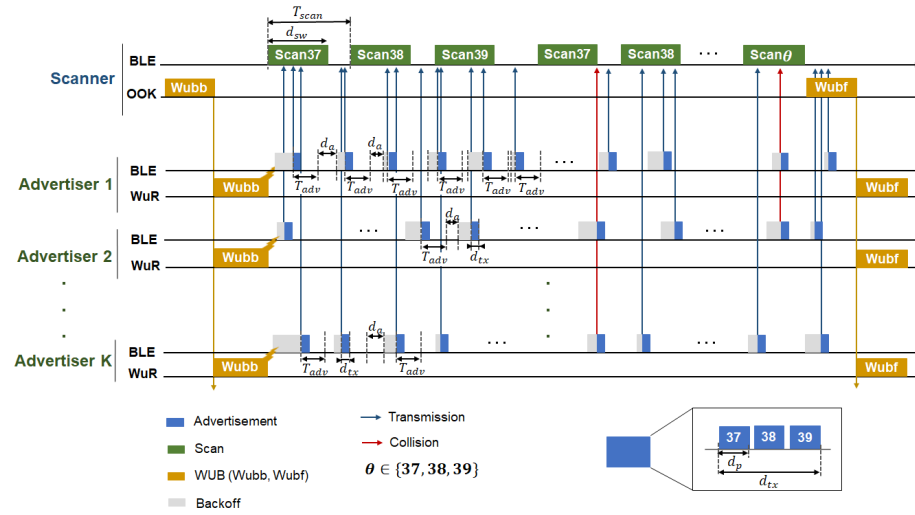
Fig. 1: WUBBLE: Neighborhood discovery protocol based on WUB ( Wubb and Wubf ).
