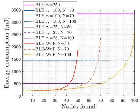
Fig. 6: Energy consumption as a function of number of nodes found w.r.t number of nodes in the network.
