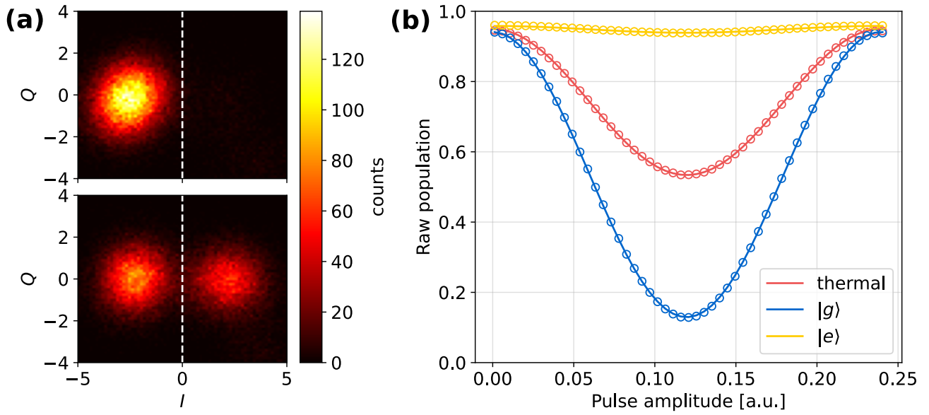
FIG. S2. (a) Histograms of the real ( I ) and imaginary ( Q ) parts of the cavity reflection coefficient, as obtained by demodulating and integrating a 600 ns pulse. The x- and y-axis have been rescaled by the standard deviation of the Gaussian envelope. Top plot is the histogram obtained when the system is initially prepared in its thermal state. Even though |g\rangle and |e\rangle are almost equally populated, the dispersive is insufficient to separate the two distributions. Bottom plot is the histogram obtained after a |g\rangle \rightarrow |h\rangle \pi -pulse. The left-blob corresponds to the |e\rangle population, unaffected by the \pi -pulse, while the right blob is due to the population transferred in |h\rangle . Setting a threshold at I = 0 (white dashed line) implements a single shot readout. (b) Calibration of the state-preparation fidelity. The qubit is prepared through sideband cooling in |e\rangle (yellow), |g\rangle (blue), or a thermal state (red). We apply a 64 ns pulse at the |g\rangle - |h\rangle transition frequency with a varying amplitude. The dynamics is then fitted using Eq. (S24) to extract the preparation fidelity (see main text for details).
