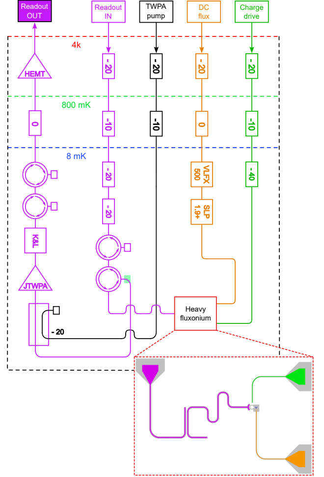
FIG. S1. Experiment schematic. The color code matches that of Fig. 1 of the main text.
