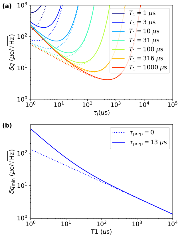
FIG. S5. Sensitivity of the heavy-fluxonium charge spectrum analyzer. (a) Charge sensitivity as a function of interrogation time \tau_I , for various qubit lifetimes T_1 (see legend). The dashed line correspond to an ideal scenario where the duty-cycle \tau_I/\tau = 1 (see Eq. (S47)). The full line corresponds to a fixed preparation/readout time \tau_{\text{prep}} = 13 \mu\text{s} . (b) Minimal sensitivity (obtained for an optimal value of \tau_I ) as a function of T_1 . The 2 scenarios considered in (a) are still represented by dashed and full lines respectively.
