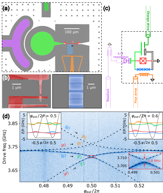
FIG. 1. Circuit diagram and implementation of the fluxonium qubit, controls and readout. Optical micrograph (a) and circuit diagram (c) of the fluxonium qubit composed of a capacitor (green), an array of 360 Josephson junctions (blue) and a single junction (red). The qubit is capacitively coupled to the readout resonator (purple). The magnetic flux through the superconducting loop can be rapidly tuned via the current passing through the flux line (orange) and the qubit is capacitively coupled to a charge line (dark green). (b) Scanning electron micrograph of the fluxonium single junction (red) and four junctions of the array (blue). (d) Two tone spectrum centered on the flux frustration point \varphi_{\text{ext}}/2\pi = 0.5 . The colorscale in the image represents the phase of the reflected probe pulse. The fit to the data (dotted lines) yields the qubit parameters E_J/h = 5.178 GHz, E_C/h = 0.4144 GHz, and E_L/h = 0.18 GHz. Central inset: detailed view of the avoided-crossing near the frustration point. The left and right insets represent the energy-level diagrams of the 4 lowest eigenstates, with the potential in grey and the wavefunctions in colors for an external flux of \varphi_{\text{ext}}/2\pi = 0.5 and \varphi_{\text{ext}}/2\pi = 0.6 respectively.
