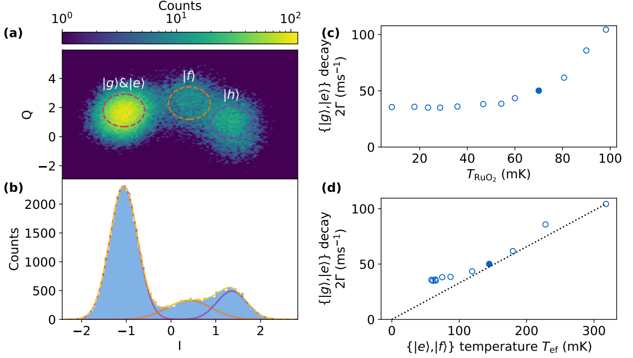
FIG. S3. Temperature dependence of the decoherence rate. (a) 2-dimensional histogram of the I, Q quadratures of the readout reflection coefficients for a qubit at thermal equilibrium with the environment. (b) Histogram of the I quadrature. The population in the manifolds \{|g\rangle, |e\rangle\} , |f\rangle and |h\rangle are determined by fitting the various peaks with Gaussian functions (see text for details). (c) Energy decay rate 2\Gamma in the \{|g\rangle, |e\rangle\} manifold measured via T_1 relaxometry (see Fig. 3a of the main text), as a function of cryostat temperature. (d) The same data are plotted as a function of the effective temperature of the |e\rangle \rightarrow |f\rangle transition, as determined from Eq. (S25). The filled point is the one extracted from the histograms in (a) and (b). The dashed line is a guide to the eyes highlighting the linear dependency above T_{\text{ef}} = 100 mK.
