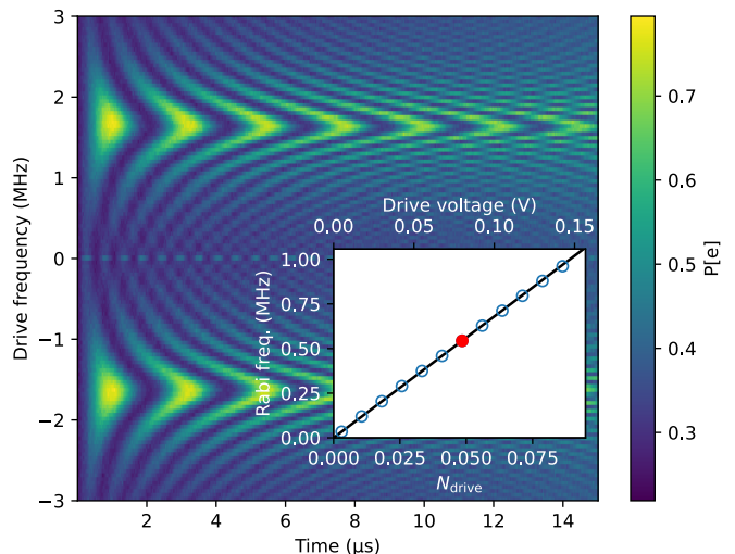
FIG. 4. Direct Rabi manipulation of the radio frequency qubit transition. after initial preparation in |g\rangle , the flux is reset to \varphi_{\text{ext}} = \pi , and the qubit is driven via the charge port with a MHz pulse of variable duration and frequency. The final qubit population is read out using the technique described in Fig. 2. The negative frequency part of the graph is here to highlight the validity range of the rotating-wave approximation. The inset shows the Rabi frequency for a resonant drive at 1.8 MHz, extracted from a sinusoidal fit, as a function of the drive voltage amplitude (upper horizontal axis). A linear fit of Eq. (5) to the data provides the lower horizontal axis calibration, where the drive amplitude is expressed in Cooper-pairs on the fluxonium electrode. The red dot is obtained for the parameters of the main figure.
