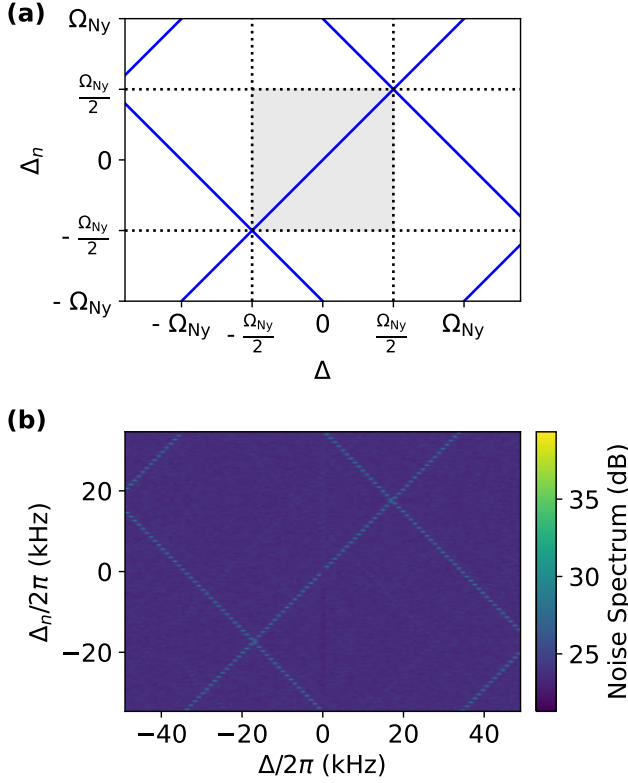
FIG. S4. Aliasing diagram of the charge spectrum analyzer: (a) The blue lines indicate the position of the peaks in discrete frequency space \Delta_n as a function of the continuous frequency \Delta of the applied tone, \Delta \equiv \Delta_n \pmod{2\Omega_{Ny}} and \Delta \equiv \Omega_{Ny} - \Delta_n \pmod{2\Omega_{Ny}} (see main text for details). (b) Experimental spectrogram with an applied tone of fixed frequency. The detuning \Delta is swept by adjusting the qubit local oscillator frequency. In this particular instance, the repetition time of the experiment was set to \tau = 14.4 \mu\text{s} , corresponding to a Nyquist frequency \Omega_{Ny}/2\pi = 35 \text{ kHz} . The frequency axis in the Figure 5c of the main text has been cropped to only display frequencies from -\Omega_{Ny}/2 \leq \Delta_n \leq \Omega_{Ny}/2 .
