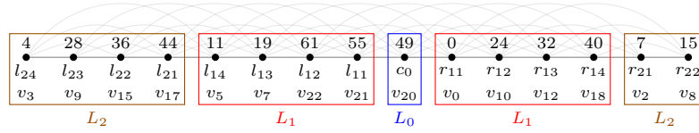
Fig. 4: Case 4. n = 14 , m = 4 , \text{diam}(P_{22}^4) = 4 , k = 6 , s = 2 .
