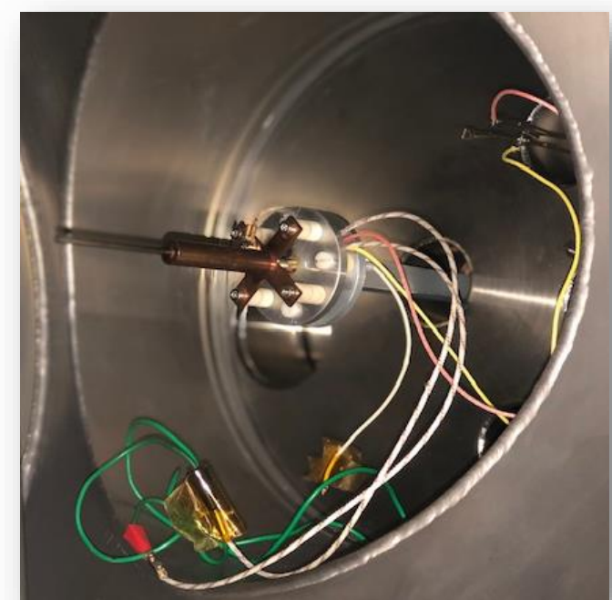
Figure 2a. Thermodesorption of aerosols.
