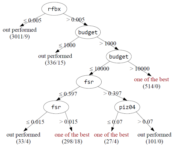
Figure 3: Decision tree for predicting when a linear penalty (LP) strategy will be one of the best strategies.
