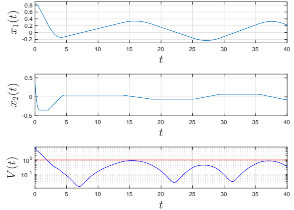
Fig. 7. Time-trajectory of the state for the system starting from x_0 = (0.8 \ 0.4)^\top and Lyapunov function V(t) in function of time.
