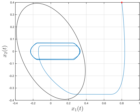
Fig. 6. Phase portrait of the system for a trajectory starting from x_0 = (0.8 \ 0.4)^\top , depicted with a red cross. The ellipsoid is the attractor \mathcal{A} , depicted in black.
