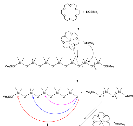
Figure 1: Postulated mechanism for polydentated ligands-silanolate catalyzed chemical recycling of silicone oil.
