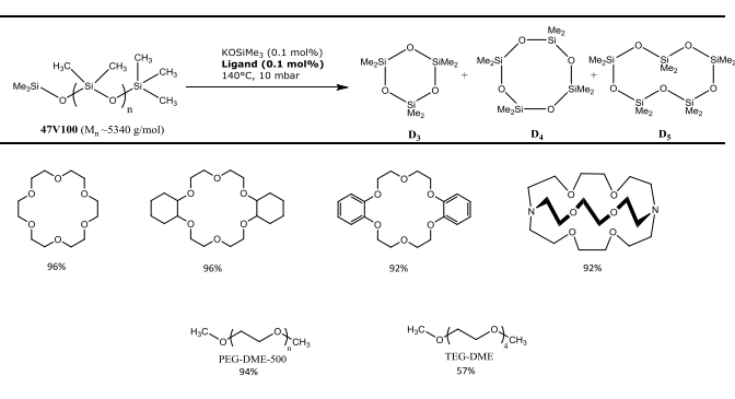
Scheme 2: Ligand screening for depolymerisation of the PDMS
