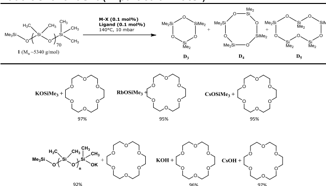
Scheme 1: Cation screening for the depolymerisation of the silicone oil.
