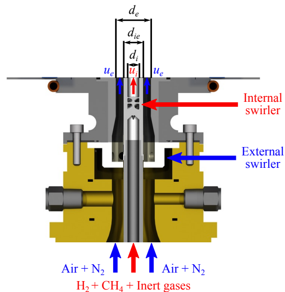
Figure 1: MIRADAS test rig equipped with the HYLON injector. In all experiments, the fuel and oxidizer channels are flush mounted with the combustion chamber backplane.
