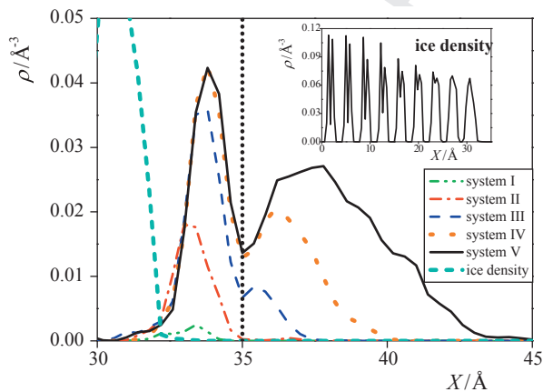
Figure 3. Number density profile of H 2 O 2 along the surface normal axis X in systems I–V. The water number density profile in system I is also shown for the outermost ice layer, and, in the inset, also for the entire system. All profiles shown are symmetrized over the two interfaces in the basic box. The dotted vertical line marks the outer boundary of the first layer of adsorbed H 2 O 2 molecules.
