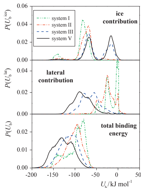
Figure 4. Distribution of the total binding energy of the first layer H 2 O 2 molecules, U_b (bottom); its contributions coming from the other H 2 O 2 molecules (middle) and from the ice phase (top), as obtained in systems I, II, III and V.
