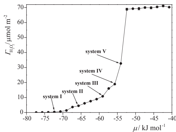
Figure 1. Adsorption isotherm of H 2 O 2 on I h ice, as obtained from our simulations. The line connecting the points is just a guide to the eye. The state points corresponding to systems I–V are marked by arrows.
