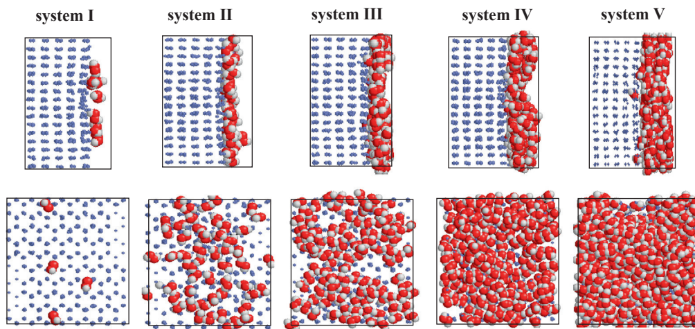
Figure 2. Instantaneous equilibrium snapshots of systems I–V, in side view (top row) and top view (bottom row). Water O atoms are shown as blue dots, H 2 O 2 O and H atoms are shown by red and white colors, respectively. Water H atoms are omitted for clarity. (For interpretation of the references to color in this figure legend, the reader is referred to the web version of this article.)
