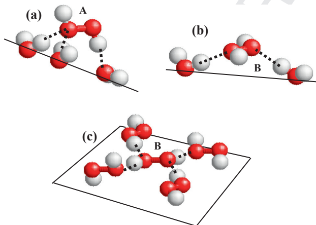
Figure 6. Possible H-bonds between a surface \text{H}_2\text{O}_2 molecule (a) in its preferred alignment A and three water molecules of the ice surface, (b) in its preferred alignment B and two water molecules of the ice surface, and (c) in its preferred alignment B and four other surface \text{H}_2\text{O}_2 molecules, also aligned in orientation B. The water orientations correspond to preferred alignments at the ice surface [6]. O and H atoms are depicted by red and white spheres, respectively, whereas the H-bonds are marked by thick dotted lines. The plane of the ice surface is also indicated. (For interpretation of the references to color in this figure legend, the reader is referred to the web version of this article.)
