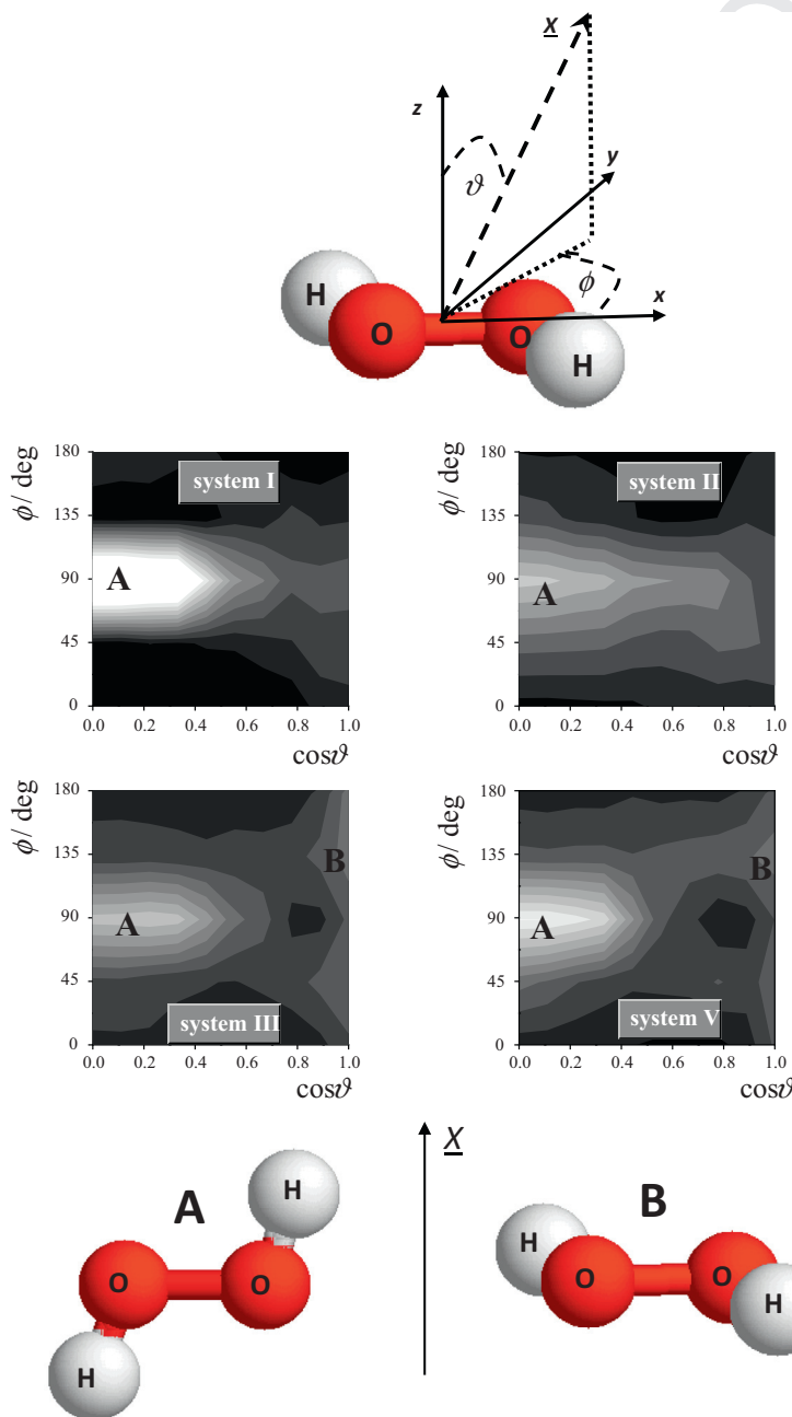
Figure 5. Orientational map of the first layer \text{H}_2\text{O}_2 molecules in systems I, II, III and V. Lighter colors indicate higher probabilities. The definition of the local Cartesian frame fixed to the individual \text{H}_2\text{O}_2 molecules (top) as well as the two preferred alignments of \text{H}_2\text{O}_2 (bottom) are also shown. \underline{X} is the surface normal vector pointing away from the ice phase.
