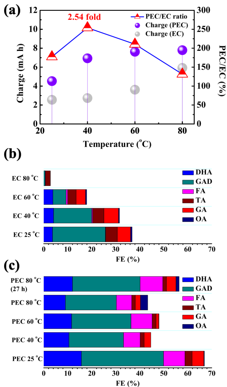
Figure 8. (a) Comparison of the charge transferred during electrocatalytic (EC) and photoelectrocatalytic (PEC) processes at 1.2 V and different temperatures (25-80 °C) as well as the enhancement PEC/EC ratio; Faraday efficiencies (FE) of liquid products in EC (b) and PEC (c) experiments. These data are associated with those shown in Fig. 6 and Fig. 7.
