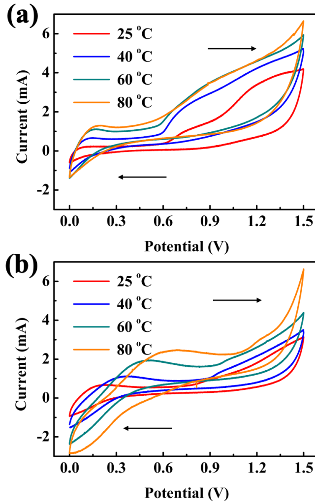
Figure 3. Cyclic voltammetry (CV) performed in the Photoelectrolyser at different temperatures (25-80 °C) under UV light irradiation ( 41 \text{ mW cm}^{-2} ) using (a) water or (b) 0.1 M glycerol as anodic solution, and water as cathodic solution. Scan rate: 10 \text{ mV s}^{-1} . The 10 th cycle is shown in each case. Anode: \text{WO}_3 /carbon cloth; cathode: Pt (20 wt.%) /C/carbon cloth; Membrane: Nafion 117.
