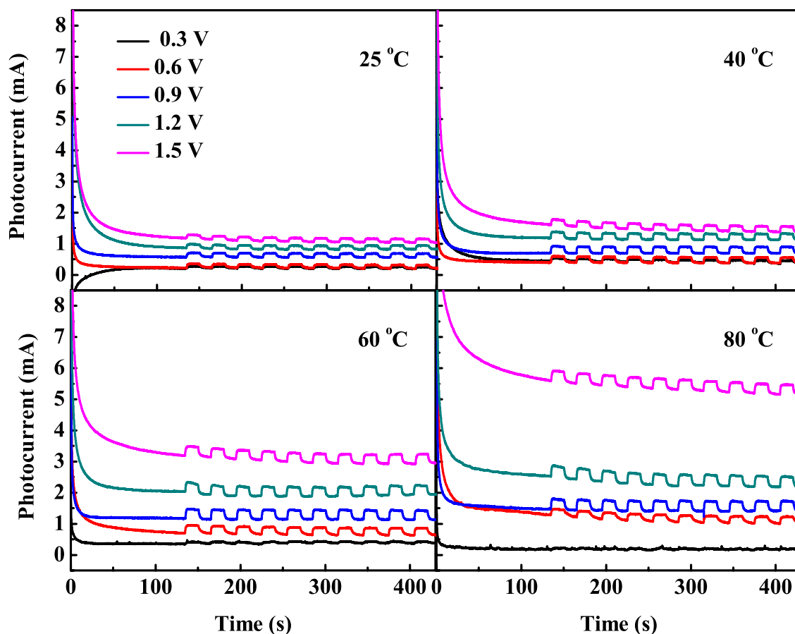
Figure 2. Transient photocurrent response at different cell voltages (0.3-1.5 V) and temperatures (25-80 °C). Anode: \text{WO}_3 /carbon cloth; cathode: Pt (20 wt.)/C/carbon cloth; Membrane: Nafion 117; anodic solution: 0.1 M glycerol (30 mL); cathodic solution: water (30 mL). Each pulse of current corresponds to an illumination of UV light pulse of 41 \text{ mW cm}^{-2} .
