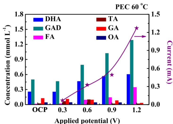
Figure 5. Influence of the cell voltage on the liquid products concentration in the anodic solution and on the obtained current after 6 h. Anode: WO 3 /carbon cloth; cathode: Pt (20 wt.%)/C/carbon cloth; Membrane: Nafion 117. Cell temperature: 60 °C. Cell voltage: open circuit potential (PC) and 0.3-1.2 V (PEC). Initial glycerol concentration in anodic solution: 0.1 M. Initial volume of anodic solution: 30 mL. UV irradiation intensity (PEC): 41 mW cm -2 .
