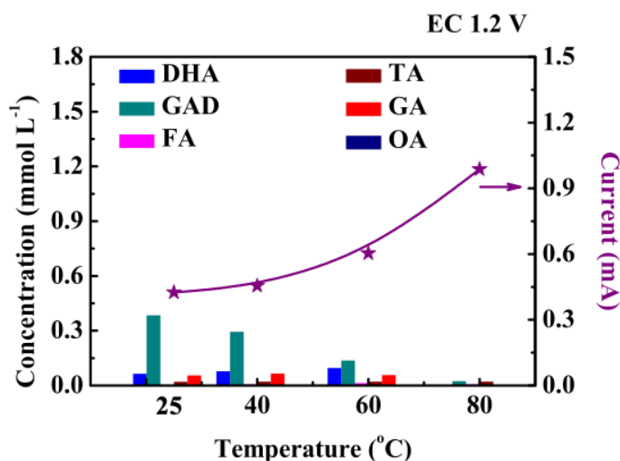
Figure 7. Influence of the cell temperature on the liquid products concentration in the anodic solution and on the obtained current after 6 h under electrocatalytic (EC) conditions (without any illumination). Anode: WO 3 /carbon cloth; cathode: Pt (20 wt.)/C/carbon cloth; Membrane: Nafion 117. Cell temperature: 25, 40, 60 and 80 °C. Cell voltage: 1.2 V. Initial glycerol concentration in anodic solution: 0.1 M. Initial volume of anodic solution: 30 mL.
