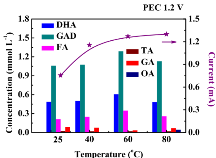
Figure 6. Influence of the Photoelectrolyser temperature on the liquid products concentration in the anodic solution and on the obtained current after 6 h. Anode: WO 3 /carbon cloth; cathode: Pt (20 wt.%)/C/carbon cloth; Membrane: Nafion 117. Cell temperature: 25, 40, 60 and 80 °C. Cell voltage: 1.2 V. Initial glycerol concentration in anodic solution: 0.1 M. Initial volume of anodic solution: 30 mL. UV irradiation intensity: 41 mW cm -2 .
