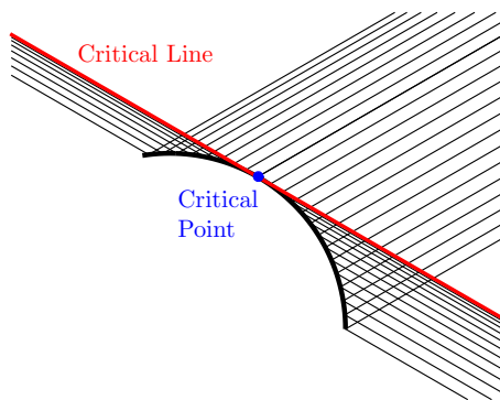
FIG. 1. Illustration of the ray accumulation on the critical line. Rays (thin black lines) are emitted from equidistant points on an arc of circle (thick black line) in the characteristic directions (here \theta = -\pi/6, \pi/6, 5\pi/6 ). The distance between consecutive rays is the smallest close to the critical line (red solid line) tangent to the surface at the critical point (blue circle).
