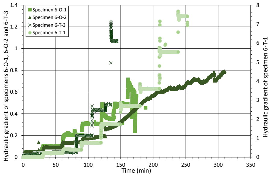
Fig. 4 Multi-stage hydraulic gradient conditions for the specimens of soil (6).
