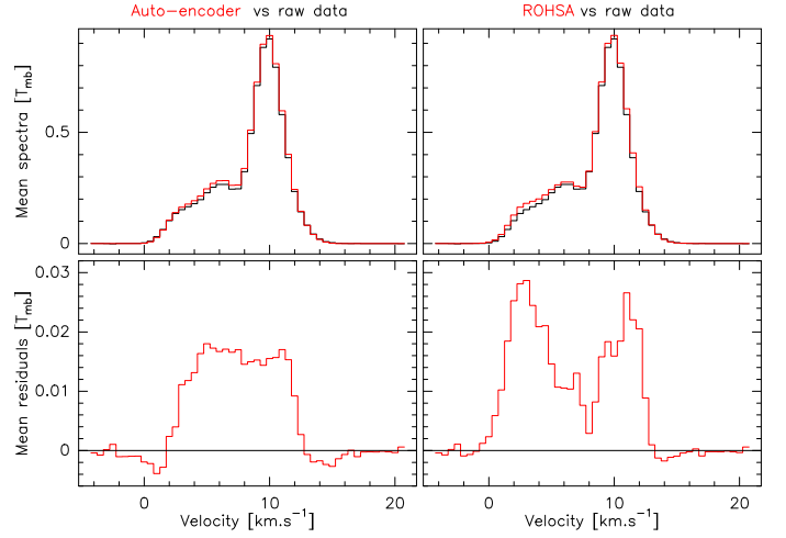
Fig. 19: Comparison of the spectral profiles and residuals for the autoencoder (left) and ROHSA (right) algorithms. Top: Comparison of the input (in black) and output (in red) intensities. Bottom: Comparison of the residuals between the input and denoised data.
