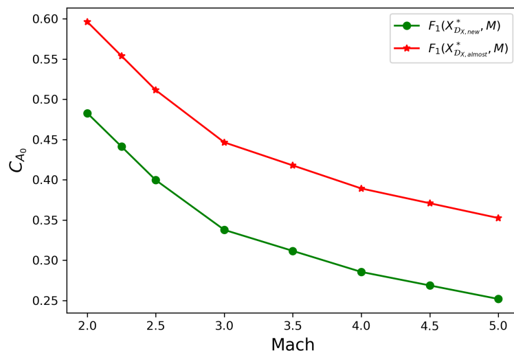
Figure 5: F_1(X, M) (evaluated with PRODAS) for characteristic values of M \in [2, 5] and for two values of X , i.e., X = X_{\mathcal{D}_{X,new}}^* (green) and X = X_{\mathcal{D}_{X,almost}}^* (red).
