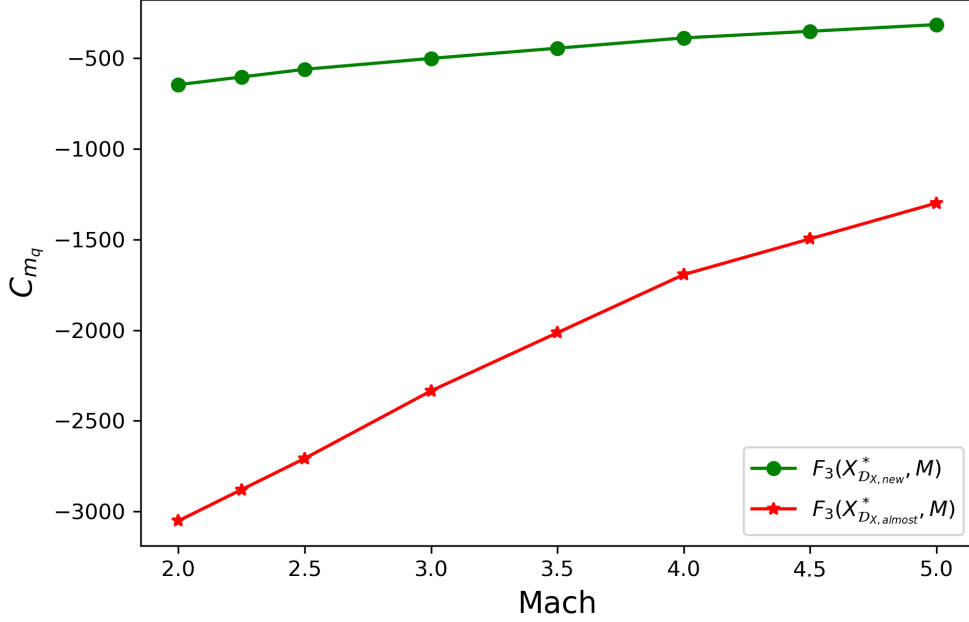
Fig. 7 F_3(X, M) (evaluated with PRODAS) for characteristic values of M \in [2, 5] and for two values of X i.e., X = X_{D_{X,new}}^* (green) and X = X_{D_{X,almost}}^* (red)
