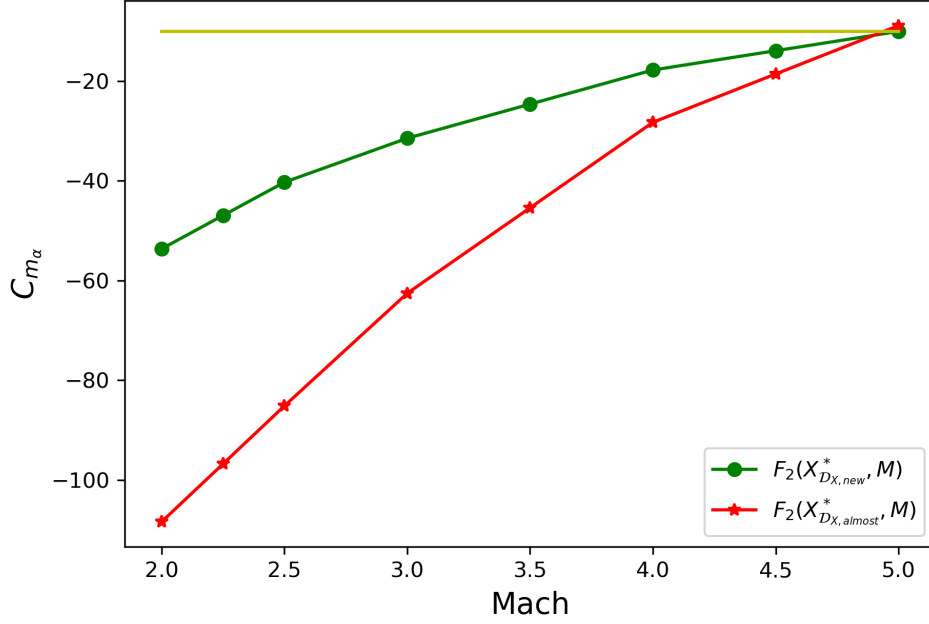
Fig. 6 F_2(X, M) (evaluated with PRODAS) for characteristic values of M \in [2, 5] and for two values of X i.e., X = X_{\mathcal{D}_{X,new}}^* (green) and X = X_{\mathcal{D}_{X,almost}}^* (red). The yellow line represents the threshold C_{m_\alpha}^{max} = -10 .
