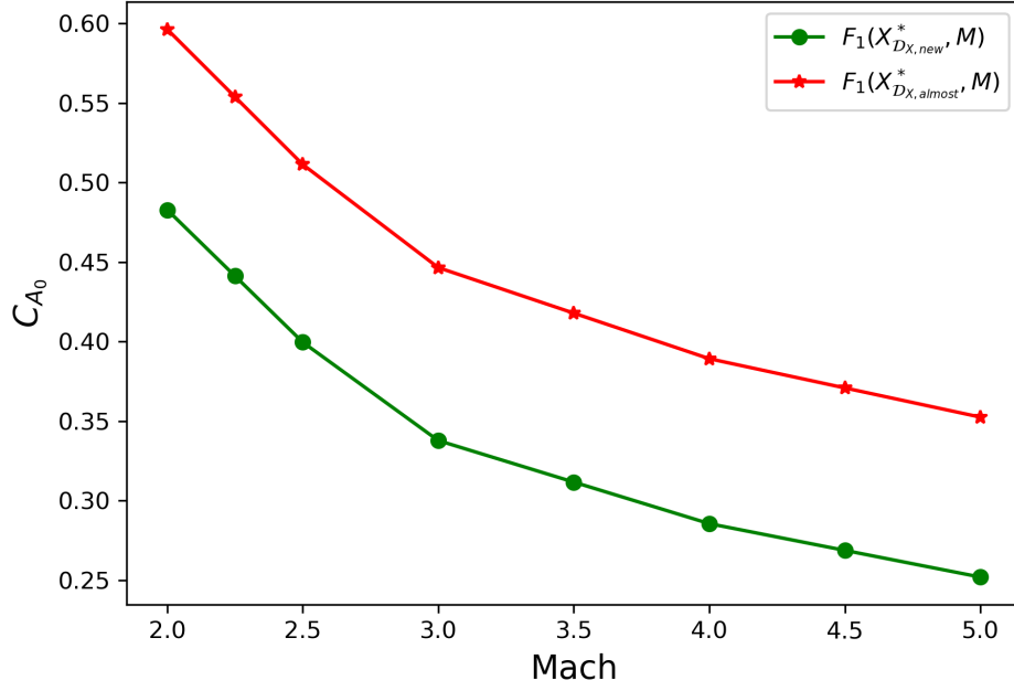
Fig. 5 F_1(X, M) (evaluated with PRODAS) for characteristic values of M \in [2, 5] and for two values of X i.e., X = X_{\mathcal{D}_{X,new}}^* (green) and X = X_{\mathcal{D}_{X,almost}}^* (red)
