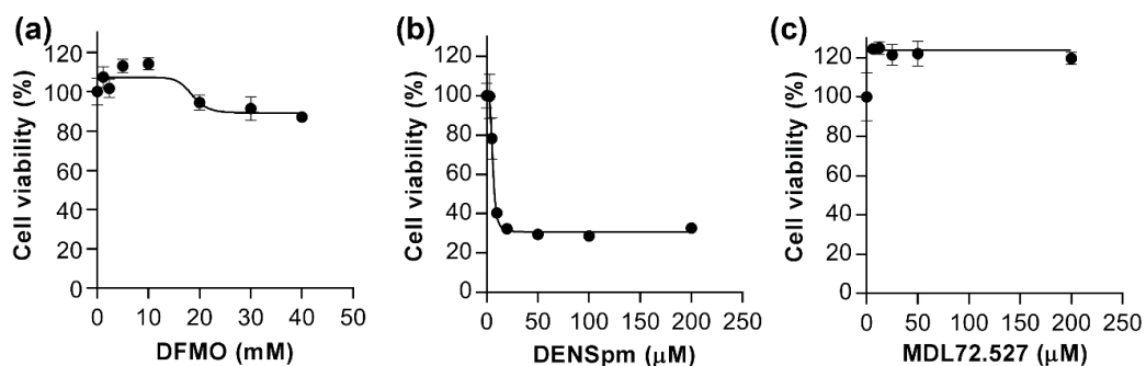
Figure 2. Toxicity of DFMO, DENSpM, and MDL72.527. Differentiated HepaRG cells were incubated with 1–40 mM DFMO (a), 3–200 μM DENSpM (b), or 6–200 μM MDL72.527 (c) for 72 h, and cell viability was assessed by standard MTT test. Results are presented as means ± S.D. from three experiments.
