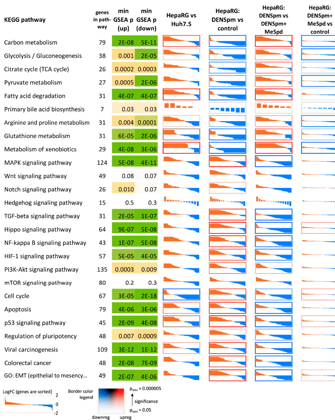
Figure 7. Differential expression profiles of genes involved in the key cell signaling pathways processes (KEGG pathways and two GO terms). Each cell represents log-transformed expression level fold changes (LogFC) of individual genes, sorted from overexpressed (red) to downregulated (blue). In each cell, vertical axis range is from LogFC = −2 (i.e., 4-fold downregulation; blue) to LogFC = +2 (i.e., 4-fold overexpression; red). Cell borders indicate the gene set enrichment test (GSEA) p -value: blue borders—enrichment with down-regulated genes, red borders—with overexpressed genes. ‘min. GSEA p (up/down)’—minimal GSEA p -value for up/down-regulated genes (across all the analyses).
