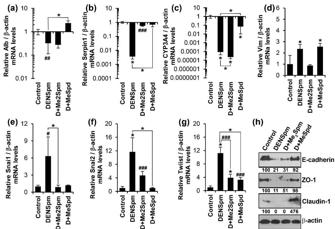
Figure 5. Metabolically-stable 3-methylspermidine and (S,S)-3,10-dimethylspermine prevent DENSpM-driven dedifferentiation of HepaRG cells. Differentiated HepaRG cells were treated for 72 h with 10 \mu M DENSpM in the absence or presence of 100 \mu M (R)-3-methylspermidine (D+MeSpd) or 100 \mu M (R,R)-1,12-dimethylspermine (D+Me2Spm). (a–g) Quantification of levels of mRNAs for liver epithelial and mesenchymal cells were performed as described above. The results are presented as means \pm S.D. from three independent experiments. * p < 0.05 , # p < 0.06 , ## p < 0.08 , ### p < 0.10 vs. untreated cells (Control) if not state otherwise. (h) Expression of claudin-1, E-cadherin and ZO-1 was quantified by western blotting, using \beta -actin as a house-keeping gene. The values represent protein/ \beta -actin levels normalized to the control (%).
