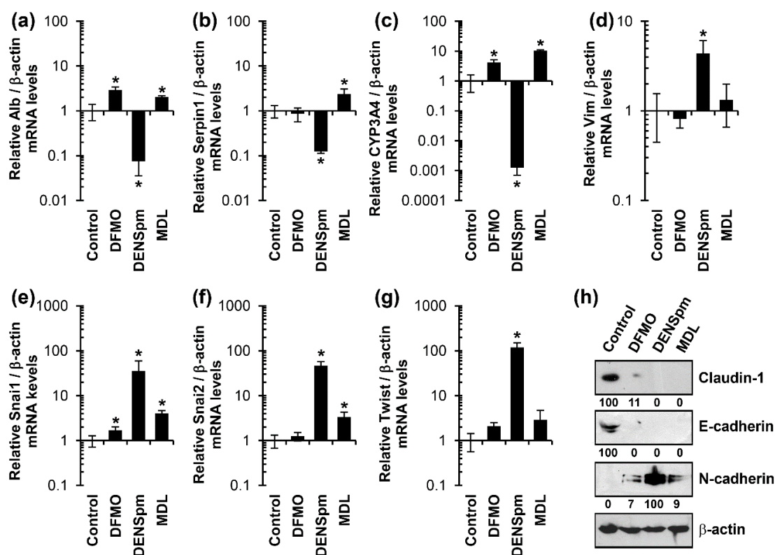
Figure 3. Diethyl-nor-spermine causes a decrease in expression of hepatocyte-specific genes and an increase in expression of mesenchymal cell-specific genes in hepatic epithelial HepaRG cells. Differentiated HepaRG cells were treated for 72 h with 5 mM DFMO, 10 \mu M DENSpm, or 25 \mu M MDL72.527 (denoted on the figure as MDL). (a–g) Quantification of levels of mRNAs for liver epithelial and mesenchymal cells were performed as described above. The results are presented as means \pm S.D. from three independent experiments. * p < 0.05 vs. untreated cells (Control). (h) Expression of epithelial (claudin-1, E-cadherin) and mesenchymal (N-cadherin)—specific genes was quantified by western blotting, using \beta -actin as a house-keeping gene. The values represent protein/ \beta -actin levels normalized to the control (%) with the exception of N-cadherin.
