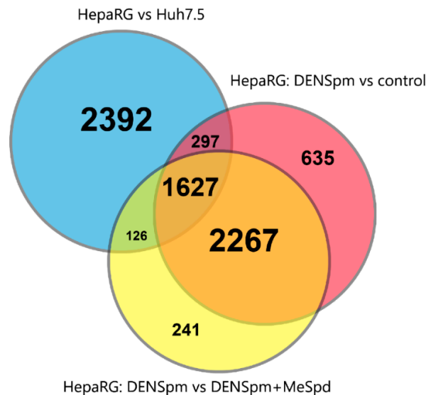
Figure 6. Venn diagram demonstrating the overlaps between the lists of differentially expressed genes for three comparisons.
