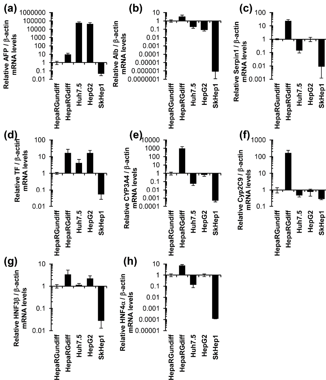
Figure 1. HepaRG cells compared to Huh7.5, HepG2 and SkHep1 cells exhibit highest expression of hepatocyte-specific genes. Expression of genes in noncancer undifferentiated (HepaRG undiff ) and differentiated (HepaRG diff ) HepaRG, hepatocarcinoma Huh7.5 and HepG2 and adenocarcinoma SkHep1 cells was assessed by RT-qPCR, and the results were normalized to the level of \beta -actin mRNA. These resulting ratios were normalized to the values obtained for undifferentiated HepaRG cells. The genes include \alpha -fetoprotein (AFP) (a), albumin (Alb) (b), \alpha -antitrypsin (Serpin 1) (c), transferrin (TF) (d) cytochromes P450 3A4 (CYP3A4) (e) and 2C9 (f), hepatocyte nuclear factors 3 \beta (HNF3 \beta ) (g) and 4 \alpha (HNF4 \alpha ) (h). Statistical analysis is presented in the Supplementary Table S3.
