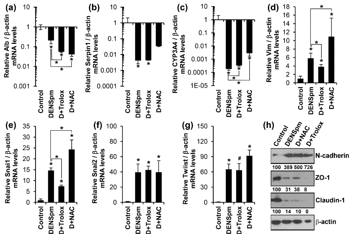
Figure 4. DENSp m -triggered dedifferentiation is not mediated by reactive oxygen species. Differentiated HepaRG cells were treated for 72 h with 10 \mu M DENSp m in the absence or presence of 100 \mu M trolox (D+Trolox) or 2.5 mM N-acetylcysteine (D+NAC). (a–g) Quantification of levels of mRNAs for liver epithelial and mesenchymal cells were performed as described above. The results are presented as means \pm S.D. from three independent experiments. * p < 0.05 vs. untreated cells if not stated otherwise (Control), # p = 0.06 vs. the untreated cells. (h) Expression of epithelial (claudin-1, ZO-1) and mesenchymal (N-cadherin)—specific genes were quantified by western blotting, using \beta -actin as a house-keeping gene. The values represent protein/ \beta -actin levels normalized to the control (%).
