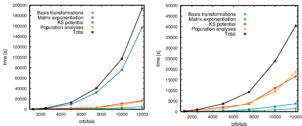
Figure 3: large water droplets containing up to 5,000 electrons are amenable to RT-TD-ADFT simulations (version 6.1.6). Timings to conduct 1 fs simulations with a time step of 50 as, PBE functional with a direct scheme to calculate electronic repulsion integrals. The x-axis represents the number of atomic orbitals. Calculations run on the Jean Zay supercomputer (at IDRIS) on 2 Intel Cascade Lake 6248 processors (20 cores per node, namely 40 cores per node, 192 GB of RAM memory and 4 Nvidia Tesla V100 16GB GPU cards. Left: Pure CPU simulations conducted with ScaLAPACK (40 CPU cores). Right: hybrid CPU-GPU simulations (40 CPUs and 4 GPUs used). Note the change of scale between the two graphs. Adapted with permission from [79] and [86].
