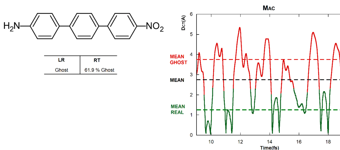
Figure 5: On the right: the CT distance ( \text{\AA} ) in the regions of the simulation corresponding to real (green) and ghost states (red). Mean CT distance considering all data points of the simulation (dashed line in black), mean CT length values derived from the ghost (dashed line in red) and real states (dashed line in green). On the left: the molecule under analysis and a table showing the result of the M_{AC}^{RT} index applied on the transition energy of the CT state predicted in the TD-DFT approach and the percentage of ghost states predicted by the M_{AC}^{RT} index in the RT-TD-DFT simulation. Reproduced with permission from [135].
