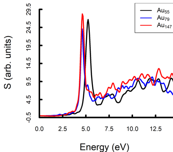
Figure 1: absorption spectra of gold nanoparticles of different sizes obtained by RT-TD-DFT simulations with deMon2k . After ITP a Dirac electronic kick of strength 0.06 a.u. was applied. RT-TD-ADFT propagations were pursued for 9 fs with a 0.001 fs time step. PBE XC functional [63] and relativistic core potentials with associated basis set have been used [64].
