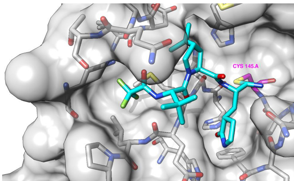
Fig 9: A) Development of Nirmatrelvir ( 73 ). H bond donors (HBD) are marked in red in the structure of PF-00835231 ( 19 ); B) Cocrystal structure of 73 bound to SARS-CoV-2 M pro (PDB: 7TE0). The nucleophile catalytic residue (here Cys145) is colored in magenta.
