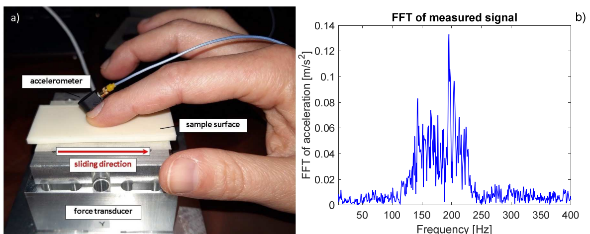
Figure 3: a) Acceleration and contact forces measurement experimental setup. The sample surface is mounted on the top of the force transducer. The FIV are measured by the accelerometer on the fingernail during the sliding of the finger on the sample surface. b) example of a frequency spectrum of a FIV signal measured on the surface sample S02.
