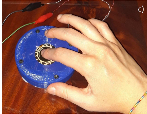
Figure 1: (a) Printed Electro-Active Polymer piezoelectric actuator; (b) Tactile rendering device PIEZOTACT, constituted by a PC for signal generation, a Texas Instruments card, and the EAP piezo actuator, fixed into an ergonomic support. (c) The tactile rendering device allows to perceive the vibration by touching the EAP actuator with the finger.
