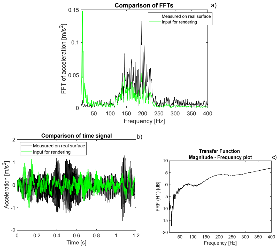
Figure 7: (a) comparison between the spectrum of the FIV measured when touching the real surface and the spectrum of the input signal to drive the tactile device. (b) comparison between the respective time signals. (c) the used Transfer Function to process the signal.
