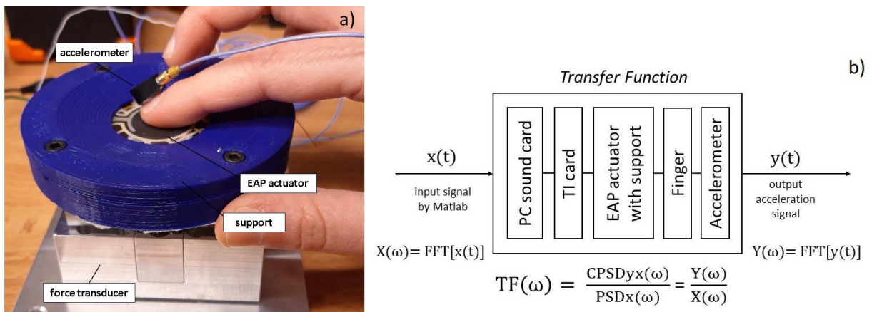
Figure 4: a) Measurement of acceleration response at the fingernail, with the fingertip in contact with the EAP piezo actuator. The actuator is mounted on the top of the force transducer. b) Definition of the Transfer Function of the system constituted by the tactile rendering device PIEZOTACT and the finger.
