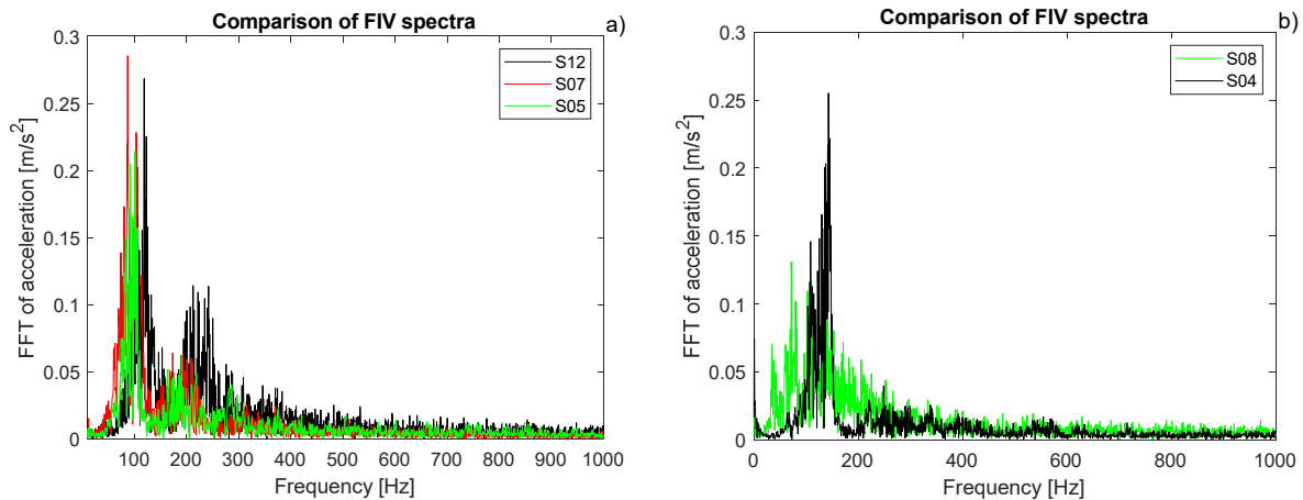
Figure 10: Examples of comparison of FIV spectra from real samples. (a) The samples S12, S07, S05 have been frequently confused in the discrimination test with both the real surfaces and the ones with simulated samples. They show similar FIV spectra; (b) the samples S08, S04 have never been confused in both the tests with real and simulated surfaces. Their FIV spectra show different frequency distribution and amplitude.
