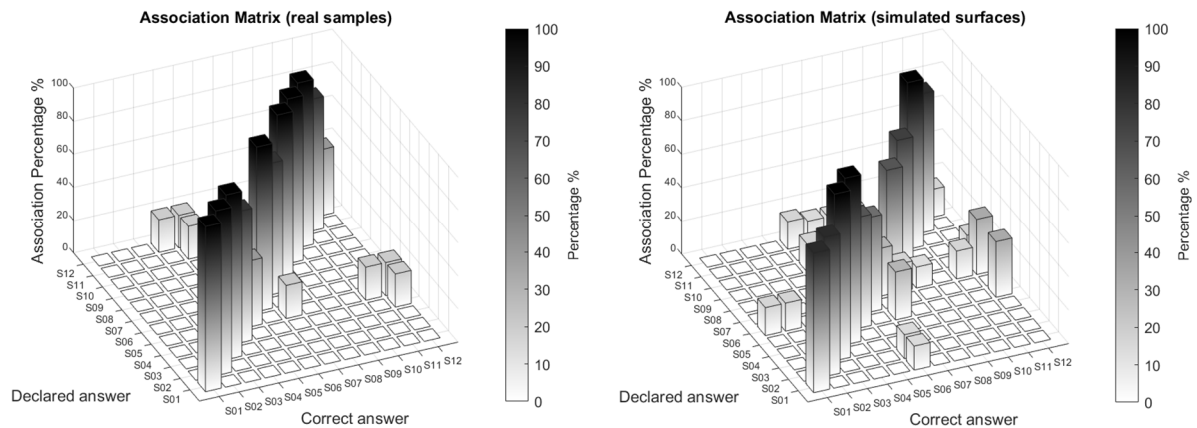
Figure 9: Results of the discrimination campaign. a) association matrix obtained with the real samples. b) association matrix obtained with the rendered surfaces with the PIEZOTACT.
