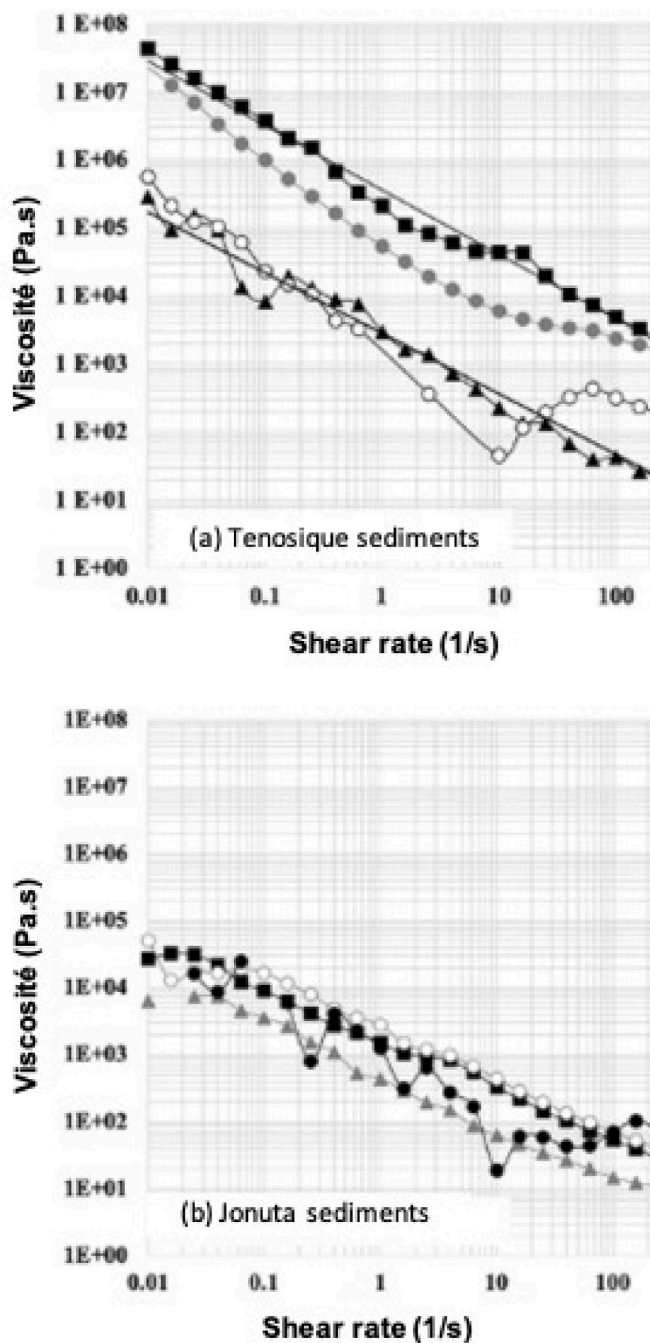
Fig. 4. Rheological behaviour of: (a) Tenosique and (b) Jonuta sediments.
