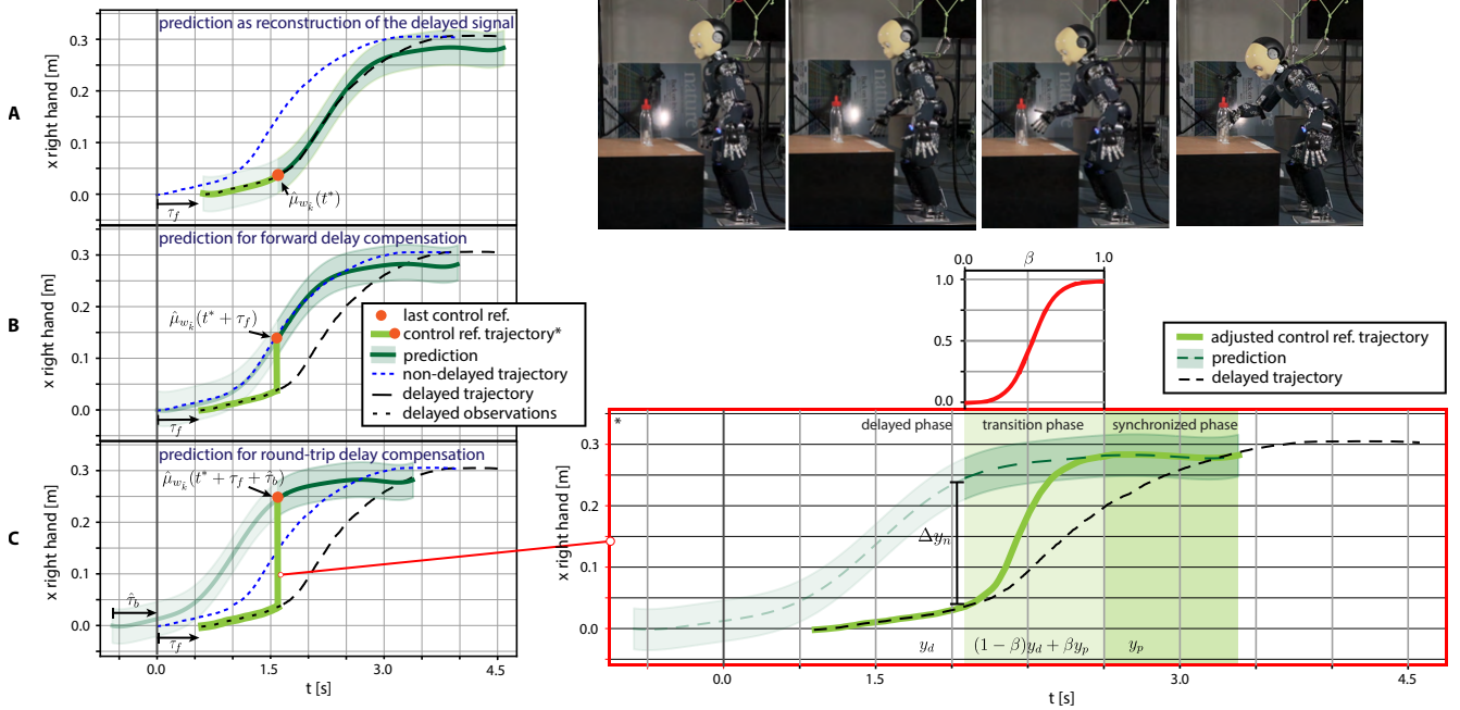
Fig. S6. Round-trip delay compensation. Given the past delayed observations, the robot produces at each time a prediction ( \hat{\mu}_{w_k} ) of the current command. To compensate for the delays, the right sample (orange dot) from the prediction has to be selected as reference for the robot controller at each time. (A) The sample corresponding to the last received observation is an estimate of the delayed command. (B) By knowing the forward delay \tau_f(t) , a sample from the prediction can be selected to achieve a synchronization between the operator’s movement and the robot movements. (C) By knowing the forward \tau_f(t) and backward delay \tau_b(t) , the robot can select the right sample from its prediction so as to achieve a synchronization between the operator’s movement and the feedback from the robot side. A policy blending arbitrates the delayed observations with the samples selected from the prediction, which guarantees a smooth transition from delayed to compensated teleoperation.
