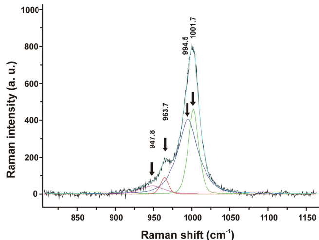
Fig. 7. Raman spectrum of yellowish hydrothermal Type 1 zircon with significant band asymmetry. Both the \nu_3 ( B_{1g} ) and \nu_1 ( A_{1g} ) modes cannot be adequately fitted with one band ( 999.7 \pm 0.8 and 967.2 \pm 1.1 \text{ cm}^{-1} with FWHM 20.3 \pm 4.2 and 25.6 \pm 4.5 \text{ cm}^{-1} , respectively), especially at the peak flanks. This particular spectrum can be satisfactorily fitted with four bands (from the right to the left: 1001.7 \pm 0.5 , FWHM 11.1 \pm 2.1 ; 994.5 \pm 0.5 , FWHM 24.0 \pm 2.8 ; 963.7 \pm 0.7 , FWHM 8.2 \pm 2.5 and 947.8 \pm 1.2 , FWHM 36.9 \pm 4.7 \text{ cm}^{-1} ). Note that despite the large uncertainties of the fit, the pairs of both modes at higher and lower wavenumbers show comparable bandwidths. The spectrum was taken in the area of point 5 in Fig. 1b. See text for further discussion.
