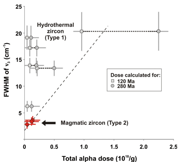
Fig. 11. Plot of the FWHM of the \nu_3 ( B_{1g} ) mode in the Raman spectra versus dose calculated from SHRIMP data ( cf. Table 2 ) according to Nasdala et al. (2001) . For hydrothermal zircon, doses for both U–Pb SHRIMP ages (120 and 280 Ma) were calculated and plotted in the figure. The points of the magmatic zircon calculated for an age of 280 Ma plot on the calibration line defined by Nasdala et al. (2001) for zircons not annealed after formation.
