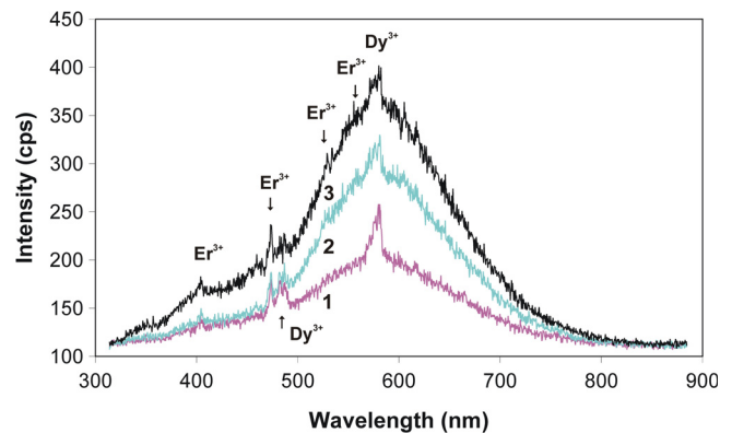
Fig. 4. CL spectra of Type 2 brownish magmatic zircon from the host rock. Spot numbers correspond to those in Fig. 2.
