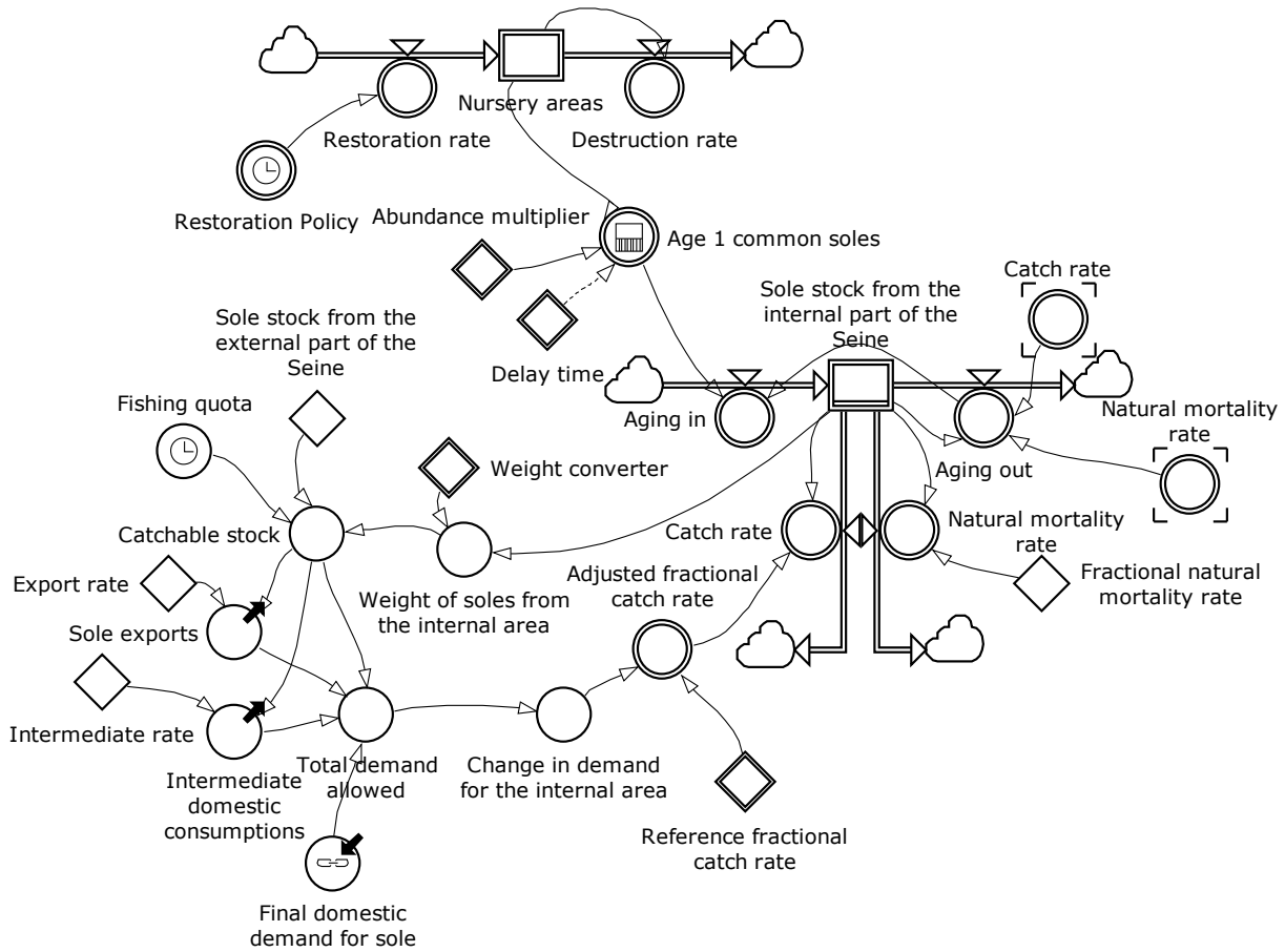
Figure 4. The global IO/SD model of the ecological system and its economic components. Boxes, double arrows, circles, and diamonds represent stocks, flows, auxiliary variables, and constants, respectively. Clouds indicate infinity and mark the model boundaries. Bold arrows into and out of auxiliary variables respectively indicate data transfer to and from the economic sub-system (in Excel).
