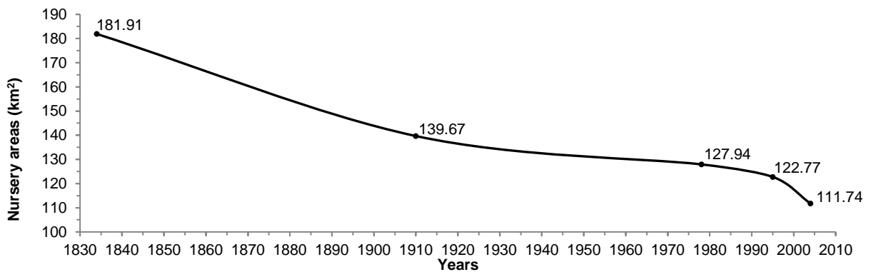
Figure 2. Evolution of nursery areas in the internal part of the Seine estuary. 3 Source of data: historical maps and habitat suitability model developed by Rochette et al. (2010).
