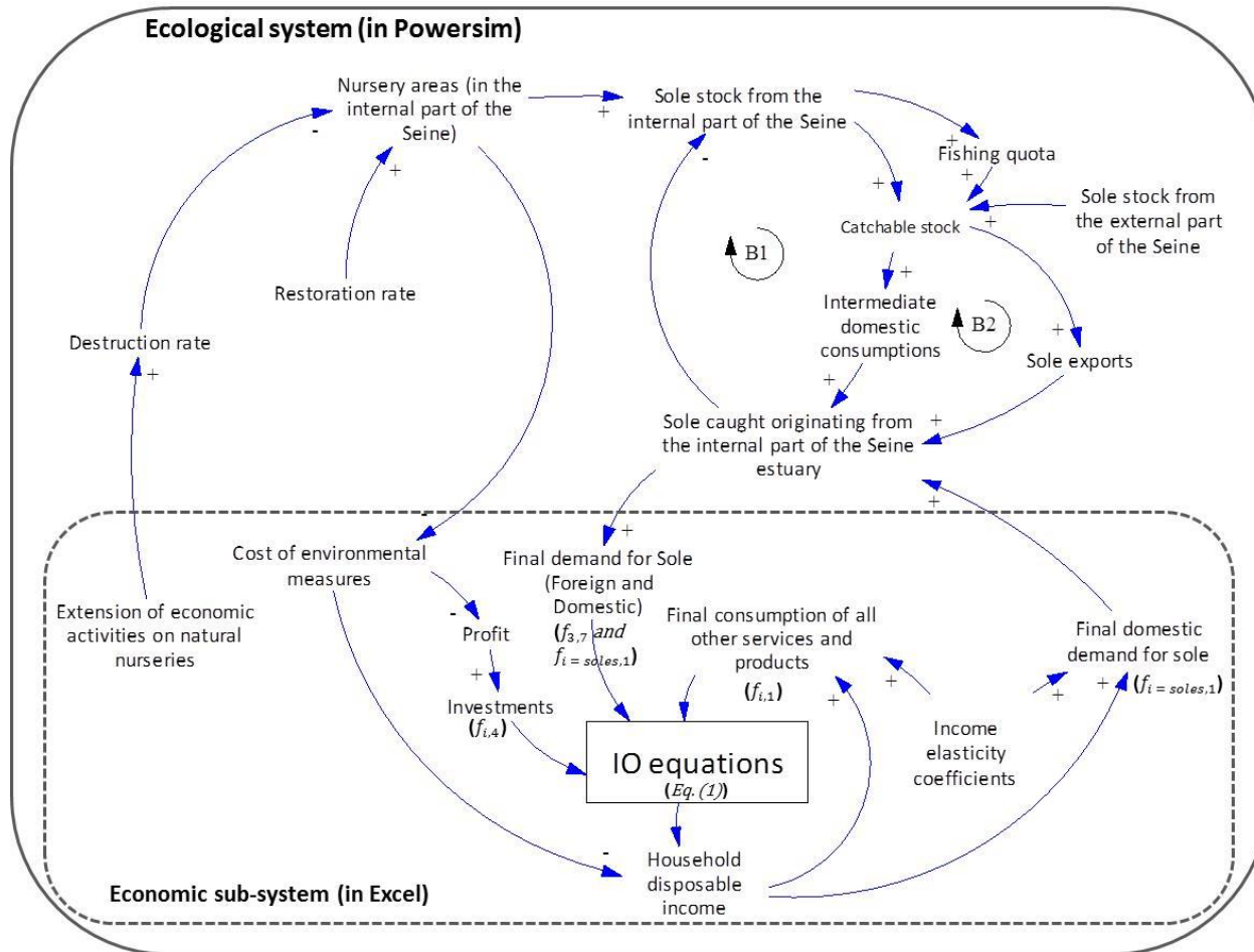
Figure 3. Interconnections between the Economic sub-system and the Ecological system “+” and “-” indicate variable changes in the “same” and “opposite” directions, respectively. The elements f_{i,k} of matrix F that connect the economic sub-system (in Excel) to the ecological system (in Powersim) are in parentheses.
