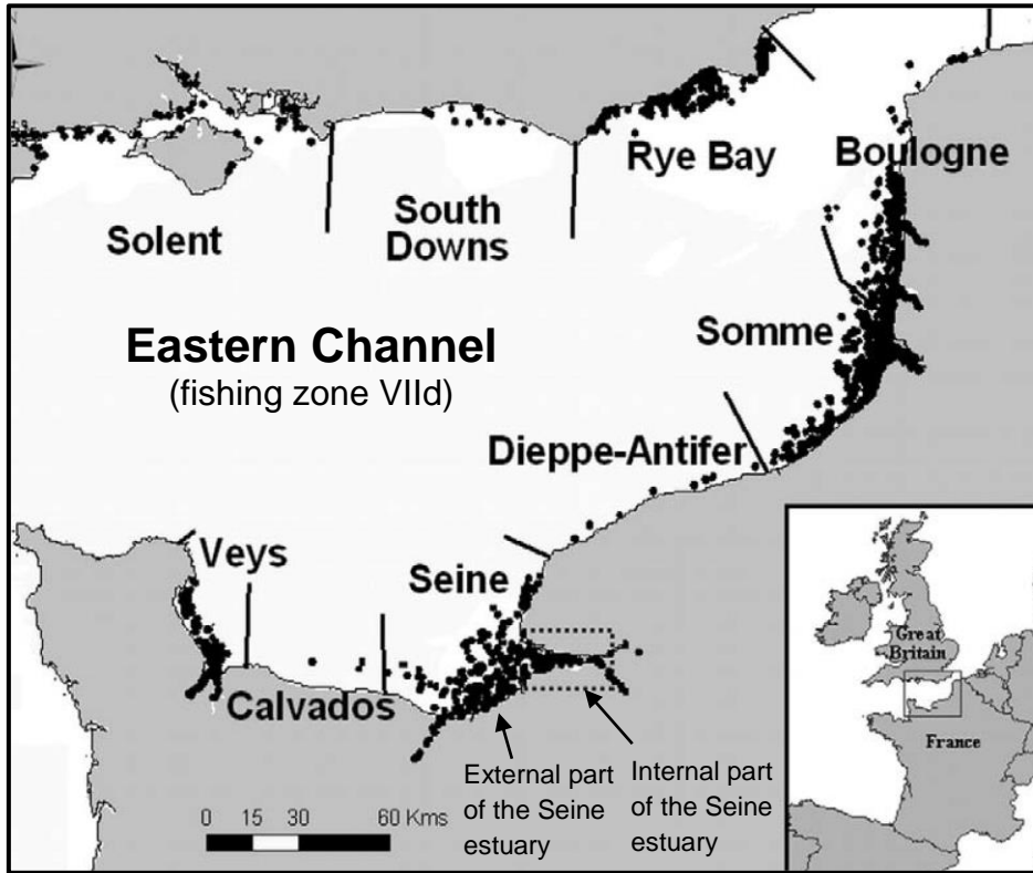
Figure 1. The Eastern Channel 2 , its sub-division into nine coastal and estuarine sectors, and the internal and external parts of the Seine estuary (inside and outside the dotted rectangle, respectively). Source of map: Rochette et al. (2010).
