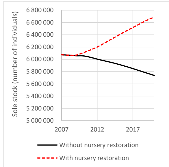
Figure 7.2 Sole stock from the internal part of the Seine estuary
