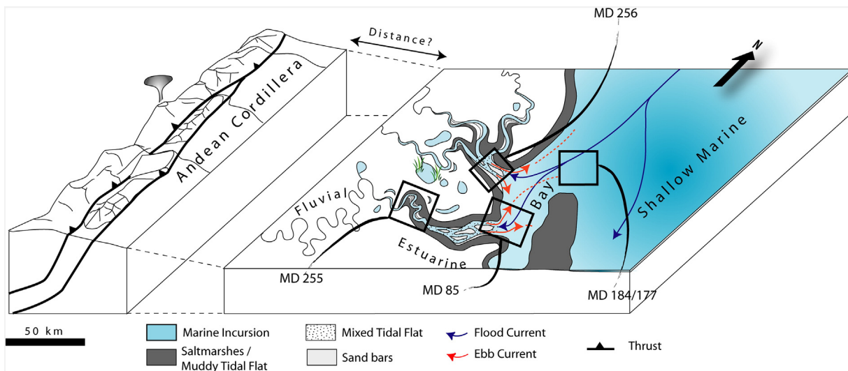
Fig. 14. Interpretative diagram for Paleocene times. Andean relief is active yet and produces sedimentary supply for the fluvial and then estuary system debouching in a shallow interior sea. Black rectangles correspond to the interpretative depositional context location of each outcrop: MD-255 corresponds to the fluvio–estuarine meandering transition zone in the proximal estuarine system; MD-256 corresponds to the inner (?) part of the estuary; MD-85 corresponds to the outer part of the estuary system and MD-184/177 corresponds to the most distal environment, also located around the outer part of the estuary system but more connected to a bay or calm confined shallow marine basin.
