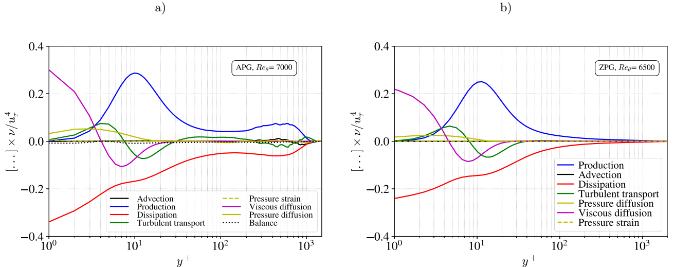
FIG. 8. Kinetic energy budget for the present APG TBL case at the streamwise position x such that Re_\theta \simeq 7000 . ( Re_\tau = 1120 ) (a) and for the ZPG TBL case of Sillero et al [22] at Re_\theta \simeq 6500 ( Re_\tau = 2000 ).
