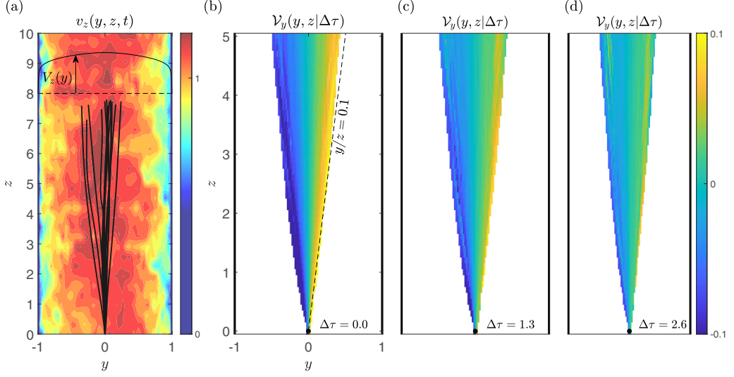
FIG. 4. (a) Instantaneous velocity v_z(y, z, t) for the channel flow simulation ( x = 0 ). The rigid walls are at y = \pm 1 . 15 fluid particle tracks injected at y = 0 , z = 0 are represented by solid lines. (b) Transverse velocity component \mathcal{V}_y(y, z | \Delta\tau = 0) based on tracer tracks with a point source seeding in a turbulent channel flow. Panels (c) and (d) are the transverse velocity maps for two positive values of \Delta\tau . \Delta\tau is a time lag introduced between velocity and position in the trajectory analysis.
