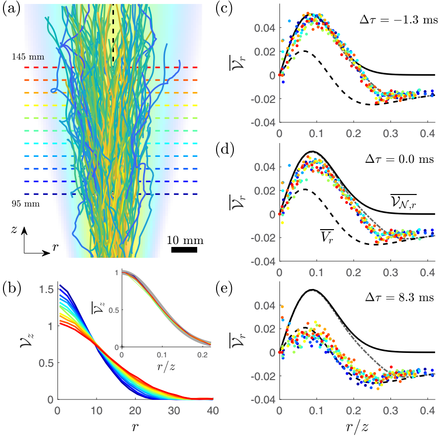
FIG. 6. (a) Particle tracks in a turbulent jet with nozzle injection. The dashed lines mark different distances z to the nozzle chosen to represent the flow profiles. (b) Axial velocity V_z obtained from the tracks analysis without time delay (standard PTV) as a function of the radial distance r for the 11 positions in z between 95 mm and 145 mm. The velocity at r = 0 decreases with increasing z . The inserted plot is the velocity normalized by the velocity at r = 0 as a function of the variable r/z . The 11 curves collapse on a master curve corresponding to the Gaussian solution (10) represented by a thick gray line. Panels (c), (d), and (e) are the normalized radial profiles \overline{V}_r = V_r(r, z|\Delta\tau)/V_z(0, z|\Delta\tau) for different values of the time delay \Delta\tau = -1.3, 0 , and 8.3 ms, respectively. The dashed line is the solution \overline{V}_r = V_r(r, z)/V_z(0, z) for the radial velocity without seeding bias [Eq. (11)]. The solid line is the solution \overline{V}_{\mathcal{N},r} = V_{\mathcal{N},r}(r, z)/V_{\mathcal{N},z}(0, z) for the tracer mean flow for a nozzle seeding [Eq. (12)]. The dash-dotted line is a model \mathcal{V}_{\mathcal{N}+\mathcal{U},r}(r, z) combining nozzle seeding and the contribution of tracers initially in the water tank [Eq. (14)].
