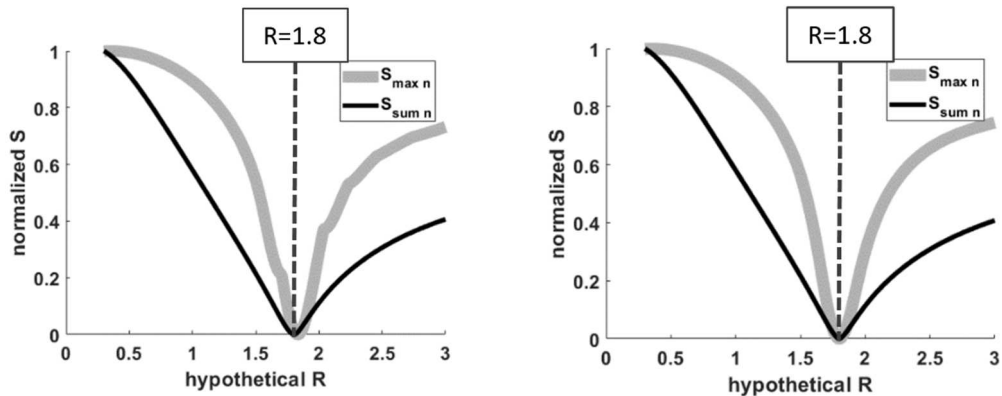
Figure 5: Evolution of S_{\max} and S_{\text{sum}} with hypothetical R for the simulated signal with R = 1.8 . Left: without zero-padding. Right: with zero-padding.
